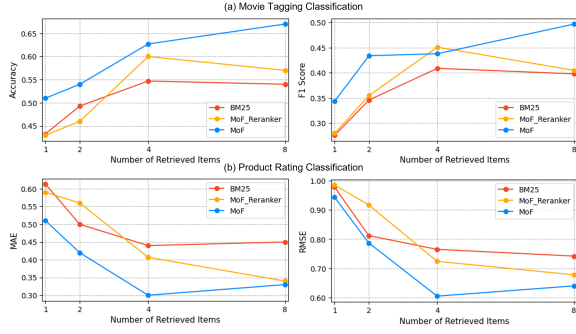
Figure 6: Impact of the number of retrieved user-history items on personalization performance. (a) shows results on LaMP-2 and (b) shows results on LaMP-3. MoF generally benefits from additional retrieved information up to moderate retrieval sizes and maintains strong performance across different retrieval sizes.
