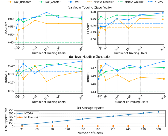
Figure 3: Scalability analysis with increasing user populations. (a), (b) show personalization performance as the number of training users increases, while (c) compares storage growth across methods.
