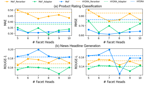
Figure 4: Impact of the number of facet heads under top-3 routing. (a) and (b) show results on LaMP-3 and LaMP-4, respectively. A moderate number of facet heads generally provides the strongest performance.
