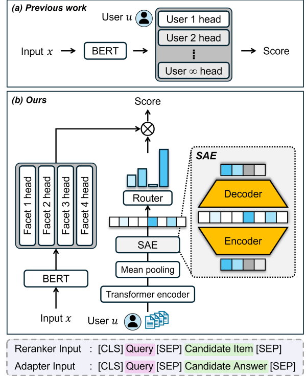
Figure 2: Comparison between (a) user-specific head personalization and (b) the proposed MoF framework. Unlike previous work, MoF combines shared facet heads through preference-aware routing.
