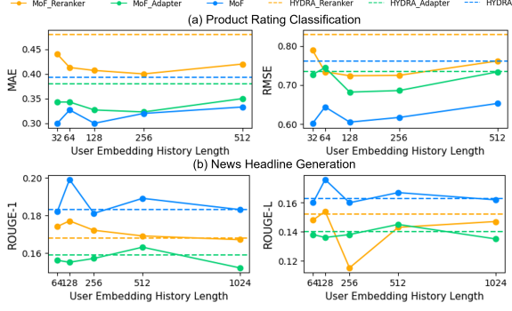
Figure 8: Impact of the number of recent user interactions used for user embedding construction on personalization performance. (a) and (b) present results on LaMP-3 and LaMP-4, respectively. Moderate history lengths generally provide stronger performance across tasks.
