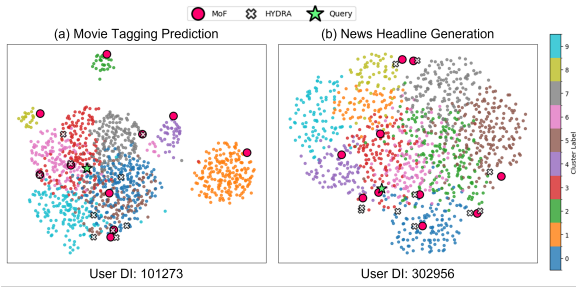
Figure 5: Visualization of CBS for two example users. Colors indicate clusters of user-history embeddings. Red circles and white crosses denote training samples selected using CBS in MoF and BM25 retrieval in HYDRA, respectively, and the green star denotes the query.
