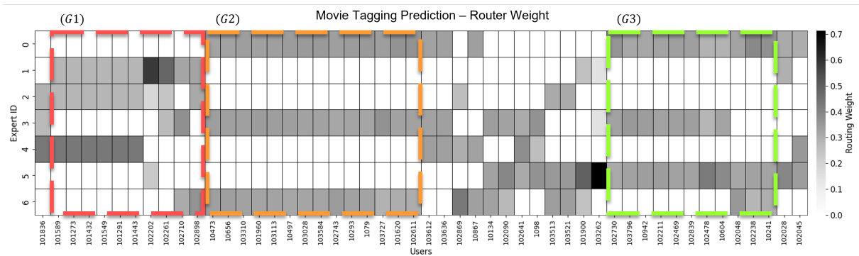
Figure 10: Heatmap of routing weight distributions across users. Users with similar routing patterns are grouped together.
