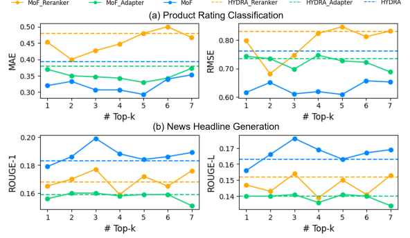
Figure 7: Impact of top- k routing on personalization performance while fixing the total number of facet heads to 7. (a) and (b) present results on LaMP-3 and LaMP-4, respectively. Performance varies with the number of activated facet heads, indicating the importance of routing selection in preference aggregation.
