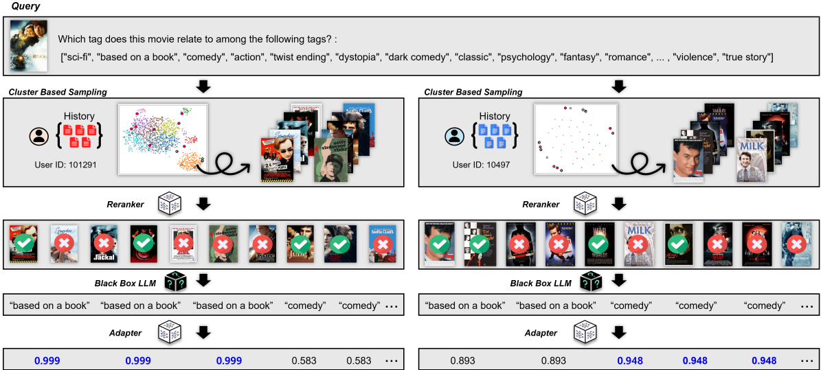
Figure 9: Case study on LaMP-2 illustrating how MoF personalizes prediction behavior for the same query. MoF selects different user-history examples and assigns distinct preference alignment scores according to each user’s tagging patterns, resulting in user-specific evidence selection and predictions.
