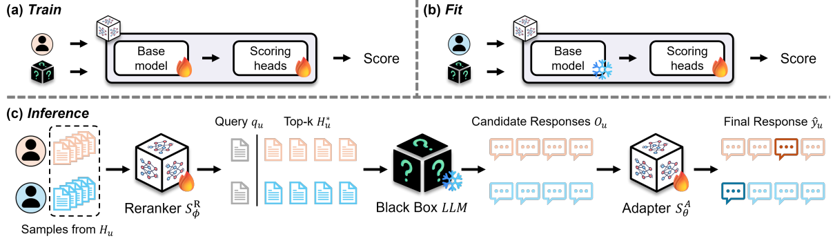
Figure 1: Overview of the training and inference pipeline. (a) Train stage: the shared base model and scoring heads are jointly trained using data collected from multiple users. (b) Fit stage: the base model is frozen while only the scoring heads are updated for unseen users. (c) Inference stage: the reranker selects useful history items, the black-box LLM generates candidate responses, and the adapter scores the candidates to produce the final response.
