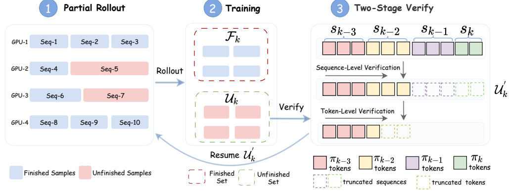
Figure 3: Overview of RollVerify. It extends the standard rollout–training loop with an additional verification phase. left: rollout phase; mid: training phase; right: proposed verification phase.
