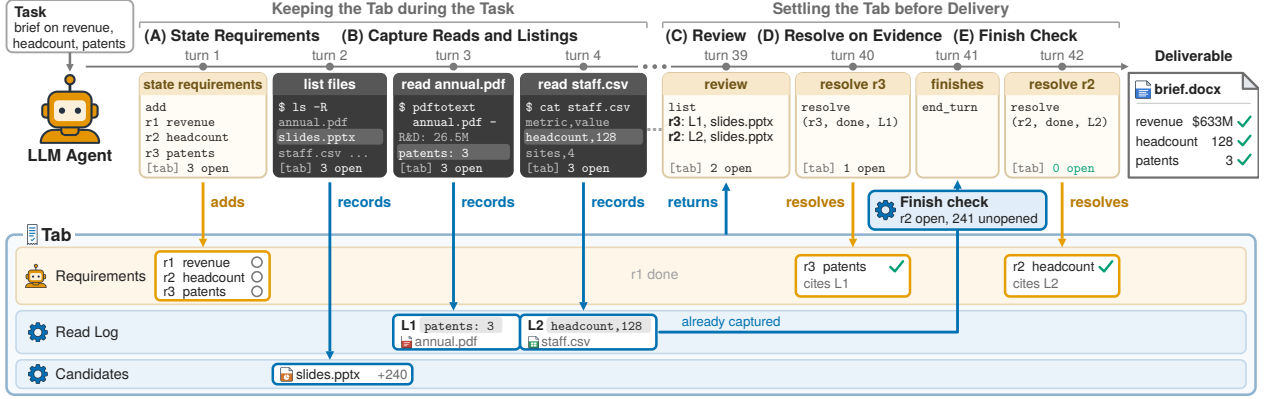
Figure 3: RunningTab over one task. The agent (top) works in turns, and the environment-side tab (bottom) fills under the turn that wrote each entry. (A) The agent states the requirements. (B) As the agent lists and reads files, the environment records each listed file as a candidate and each read as a read log entry with its anchor. (C) The review shows each open requirement beside its best read log match and the unopened files. (D) The agent resolves a requirement by citing the read log entry that holds its content. (E) At the stop, the environment returns one finish check with what is still open; here the tab had already captured the missing fact, so the agent closes it and delivers.
