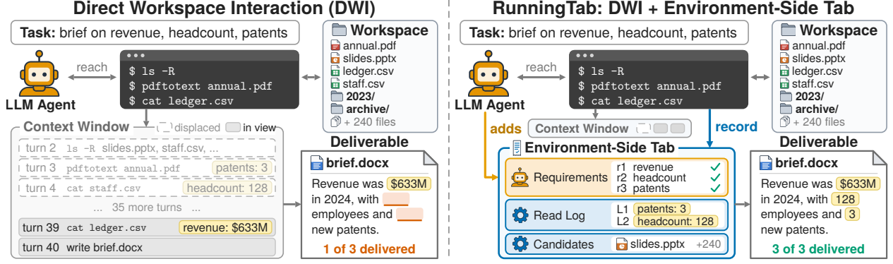
Figure 1: Direct workspace interaction (DWI) and RunningTab on an illustrative task: a brief that needs three facts scattered across a workspace. (Left) In DWI, the agent reaches every file through its terminal, but what it reads lives only in its context window: facts read early are displaced by later observations, and the brief is delivered without them. (Right) RunningTab keeps an environment-side tab beside the agent: the agent adds the requirements of the task, the environment records what is read and what is listed but not opened, and the facts remain available until the deliverable is written.
