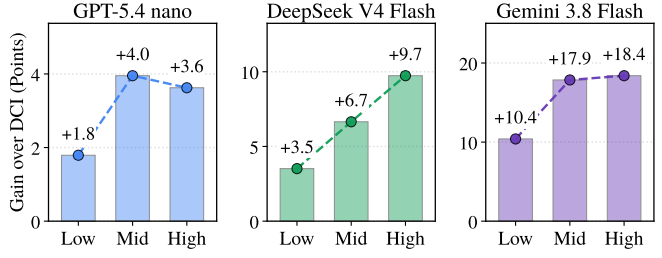
Figure 5: Gain of RunningTab over DCI in Pass Rate on tasks split into thirds by how much the agent reads.
