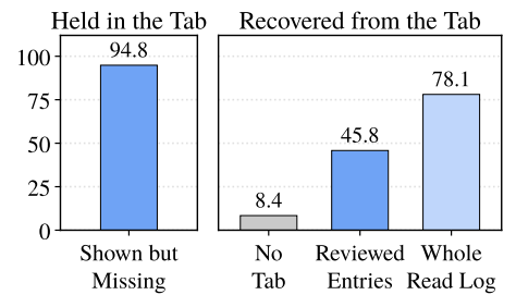
Figure 4: RunningTab with GPT-5.4 nano on Workspace-Bench (%). (Left) Values held in the tab, among those the agent was shown but its deliverable lacks. (Right) Held values that an LLM recovers when they are masked, by the part of the tab given.
