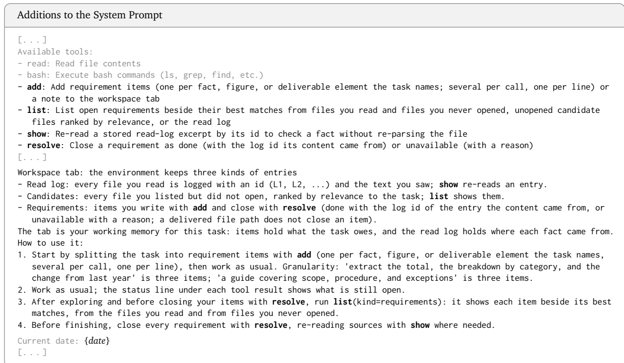
Figure 6: Additions of RunningTab to the system prompt (Section 3.3). Text in gray is the system prompt of the harness, shown only to locate the additions, with [...] marking omitted parts.
