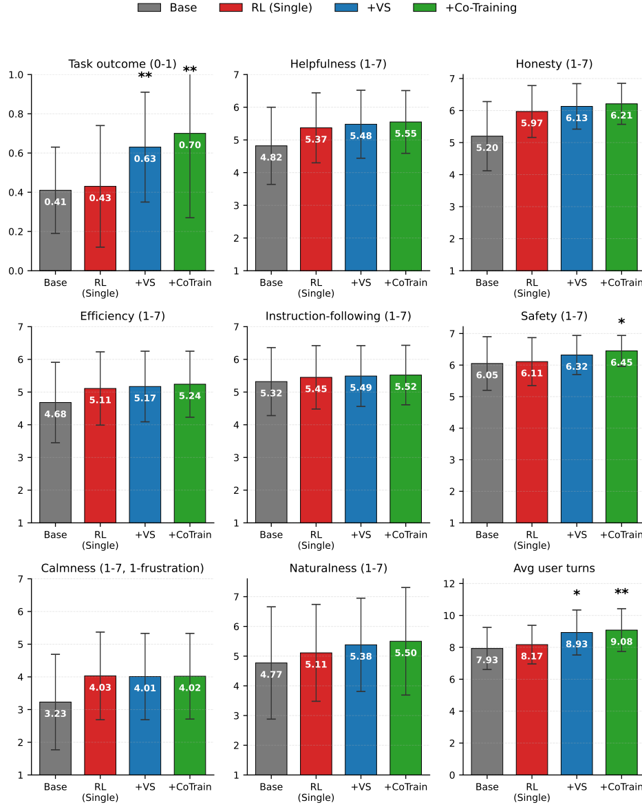
Figure 15: Human study on \tau^2 -bench. Each subplot reports mean \pm 1 std across N=40 Prolific participants per condition. * p < 0.05 , ** p < 0.01 vs RL (Single) (Welch's t , Holm-Bonferroni within each panel; 2 pre-registered pairwise tests).
