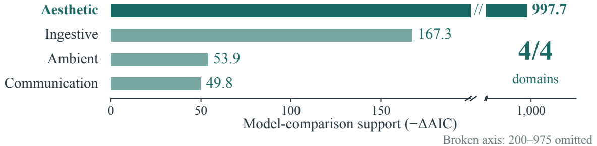
Figure 6: Signed movement, not endpoint-only extremity. Bars show -\Delta\text{AIC} for the \text{gate} \times \text{direction} account against the extremity-only (ERS) account in the dense two-model audit, from the mixed-model fit with crossed item and model components reported in this appendix. Larger positive magnitudes favor the signed account; all four domains do so (ingestive is coded ambiguous; Table 9). The linear axis omits 200–975, with the break explicitly marked.
