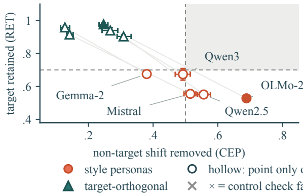
Figure 8: Prespecified robustness and boundary checks. (a) Interval-bound rank and band cells on the seven-point readout: circles denote the style-persona subspace and triangles the constructed target-orthogonal subspace; filled symbols clear the required 95% bound, hollow symbols pass only at the point estimate (in b, fail the control check), and crosses fail the control check; cell shading marks where the subspace clears the bound. (b) Binary-readout CEP–RET with item-paired intervals. Filled symbols identify the sole model that passes the control check; hollow points remain descriptive. (c) Collateral-utility checks for the constructed subspace; only Mistral passes all five.
