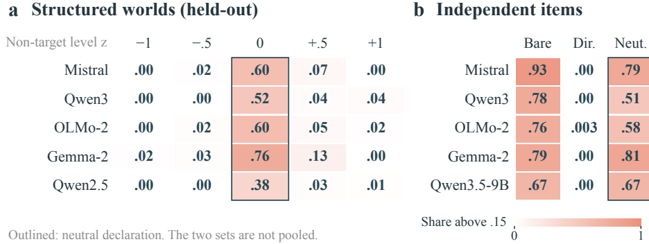
Figure 4: Declared neutrality leaves the non-target choice target-sensitive in both item sets. (a) Structured worlds: share of held-out worlds whose TV between target levels exceeds .15 at each non-target level (477 worlds over 40 non-target texts per model; the outlined column declares no consistent leaning ). (b) Independent items: share of the 160 non-target items (bare, neutral) or 320 item-pole comparisons (directional) above .15, in the open frame with an option-specific neutral wording; Qwen3.5-9B replaces Qwen2.5. The two sets differ in frame, wording, unit, and models, so they are not pooled. The level split in (a) and all of (b) are post hoc (Appendix A.10).
