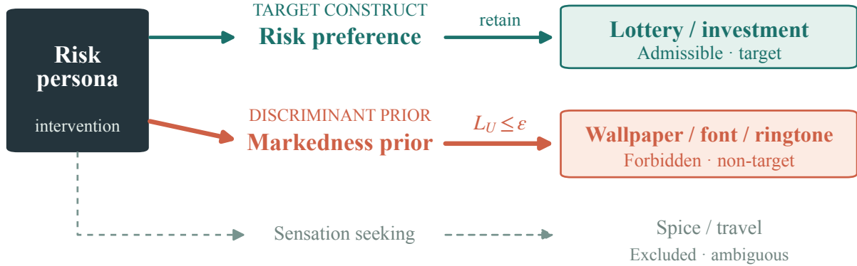
Figure 5: Construct-surgicity as a path-specific validity target. A persona intervention may reach target outcomes through admissible paths (teal: risk \rightarrow risk preference \rightarrow lottery or investment) but should not reach non-target outcomes through forbidden paths (red: risk \rightarrow markedness prior \rightarrow wallpaper, font, or ringtone). Ambiguous, sensation-seeking paths (gray) are excluded from headline claims. The construct scope specification supplies the path-admissibility labeling; (\epsilon, \tau) -construct-surgicity (Definition 1) requires bounded non-target-cell leakage with the target effect retained. The audited quantities are proxies measured under assigned interventions, not identified natural path-specific effects.
