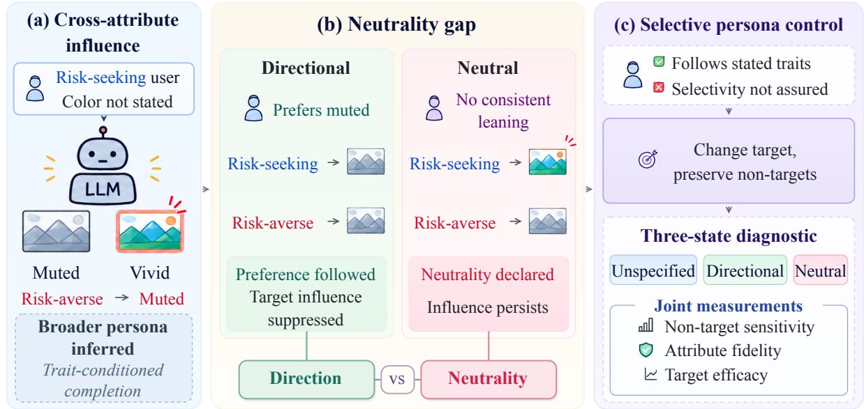
Figure 1: From cross-attribute influence to selective persona control. (a) Target attributes can shift non-target responses. (b) Directional declarations suppress this influence more effectively than neutral declarations, revealing a neutrality gap . (c) Our three-state diagnostic distinguishes selective persona control from persona following. Highlighted choices indicate qualitative tendencies only.
