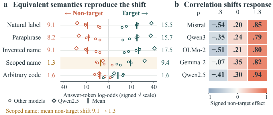
Figure 2: Equivalent semantics reproduce the shift, and supplied correlations redirect it. (a) Answer-token log-odds relative to the no-information reference (no stated preferences), on non-target and target items under five wording conditions; “Scoped name” replaces the examples with a risk-only scope. Points are the five checkpoints (diamonds: Qwen2.5); ticks and numbers give their means. Non-target values are mirrored leftward on a signed-square-root axis. (b) Signed effect of the bare prompt on the semantically positive non-target option at each demonstration correlation \rho (64 shared worlds; means and intervals in Appendix A.8; Gemma-2’s negative- \rho interval includes zero).
