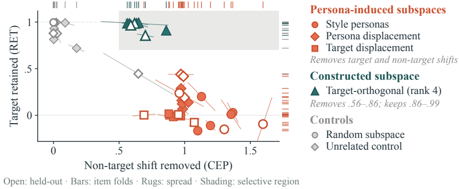
Figure 3: Persona-induced subspaces remove target and non-target shifts together. Non-target shift removed (CEP) against target response retained (RET) after erasure, on the five primary and three held-out checkpoints. Persona-induced subspaces are fit to the style personas’ contrast, the risk persona’s own displacement, or its displacement on target items. Of those plotted, only the constructed target-orthogonal subspace enters the selective region (shaded; \text{CEP} \geq .5 , \text{RET} \geq .7 ).
