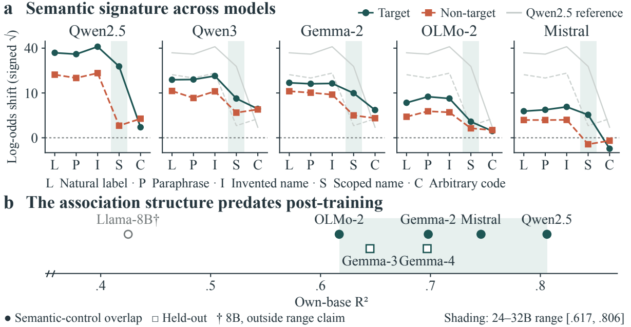
Figure 7: Semantic signatures and own-base prediction. (a) Target (circles, solid) and non-target (squares, dashed) log-odds shifts for each checkpoint in Figure 2a. Pale curves repeat Qwen2.5; the common signed-square-root scale retains original-unit tick labels and negative values. L, natural label; P, paraphrase; I, invented name; S, scoped name (risk-only scope, no examples); C, arbitrary code. Lines guide comparisons between categorical conditions; shading marks S. (b) Own-base R^2 for seven base–instruct pairs. Filled circles overlap the semantic-control checkpoints; open squares are the Gemma-3 and Gemma-4 pairs, and the hollow circle is the Llama-3.1-8B pair. Vertical separation distinguishes groups only. The shaded 24–32B primary-panel range [.617, .806] is not a confidence interval; Llama-3.1-8B is outside that scale claim. The axis starts at .35.
