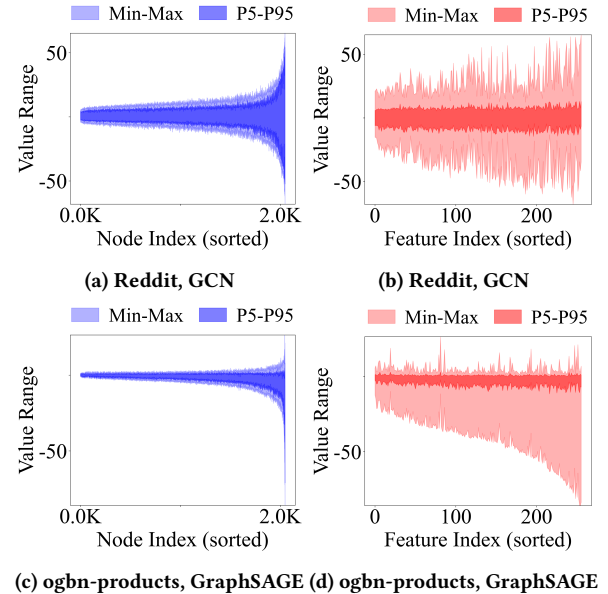
Figure 2: Node-wise(blue, left) and feature-wise(red, right) range plot, sorted in ascending order. ‘Node Index’ indicates each node, and ‘Feature Index’ indicates each feature dimension. Each plot shows the min-max range and the 5th-95th percentile range of the values within the same dimension.
