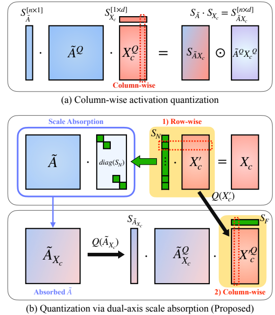
Figure 3: Comparing quantization at aggregation phase.
