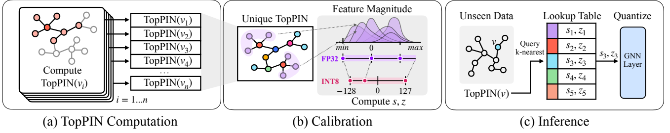
Figure 4: Quantization process with TopPIN. (a) shows node group generation through the proposed topological proxy, TopPIN. Each color is used to denote each group. (b) shows the calibration process to obtain quantization parameters for each group. (c) demonstrates how inference is done on unseen data, using the quantization parameters of the nearest groups with interpolation.
