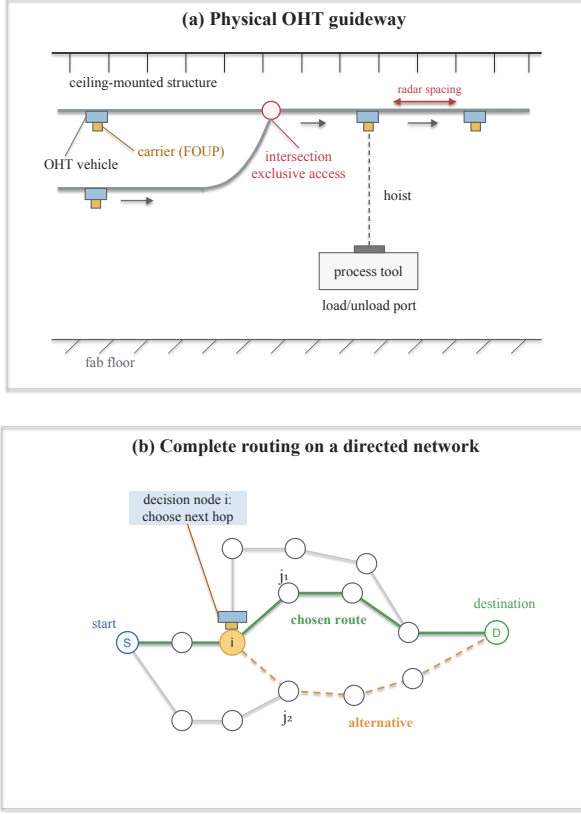
Fig. 1. OHT routing context and decision process. (a) Vehicles move carriers along a ceiling-mounted, unidirectional guideway where safety spacing, shared segments, and exclusive intersections couple travel times across the fleet. (b) On the directed guideway graph, an OHT with destination D makes a local next-hop decision at split node i , choosing between candidates such as j_1 and j_2 , and repeats these decisions to form a complete route from start to destination.
