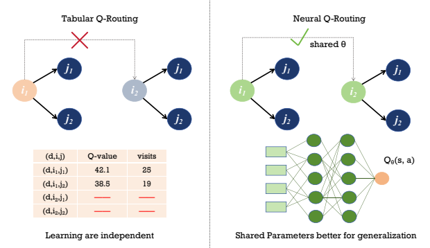
Fig. 2. Tabular versus neural Q-routing. Tabular Q-routing stores an independent value for each (d, i, j) tuple, whereas a neural value function Q_\theta(s, a) scores candidate actions from a common state-action feature vector \phi(s, a) . Shared parameters let observations from frequently visited contexts inform the fitted scoring rule used at less frequently visited contexts.
