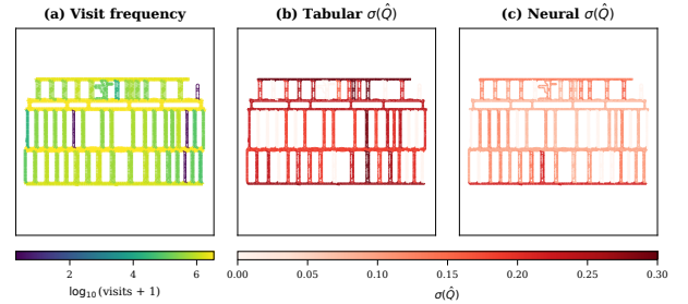
Fig. 7. Value-estimate stability of tabular and neural Q-routing on the fab guideway of Fig. 3. All panels use the same layout, with color aggregated by bay. (a) Visit frequency of (d, i, j) tuples. (b) Standard deviation of tabular estimates over the final snapshots. (c) Standard deviation of neural estimates over the same snapshots.
