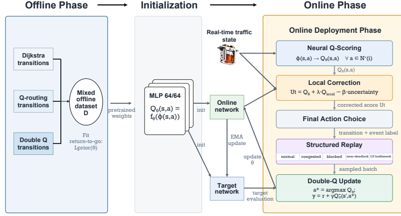
Fig. 4. Method overview. Logged trajectories initialize the online and target value networks. During operation, Double-Q updates refine the shared value function, while a local congestion correction adjusts action rankings from recent edge-level observations and event-stratified structured replay retains predefined congestion and service-event classes.
