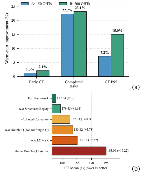
Fig. 5. Warm-start and component analyses. (a) Relative warm-start improvement over cold start during the first 200 s; Early CT is the mean CT of tasks completed in that interval. (b) CT Mean for the neural component deletions and the tabular Double-Q baseline; parentheses report the difference from the full framework. The panels visualize Tables III and IV, respectively.
