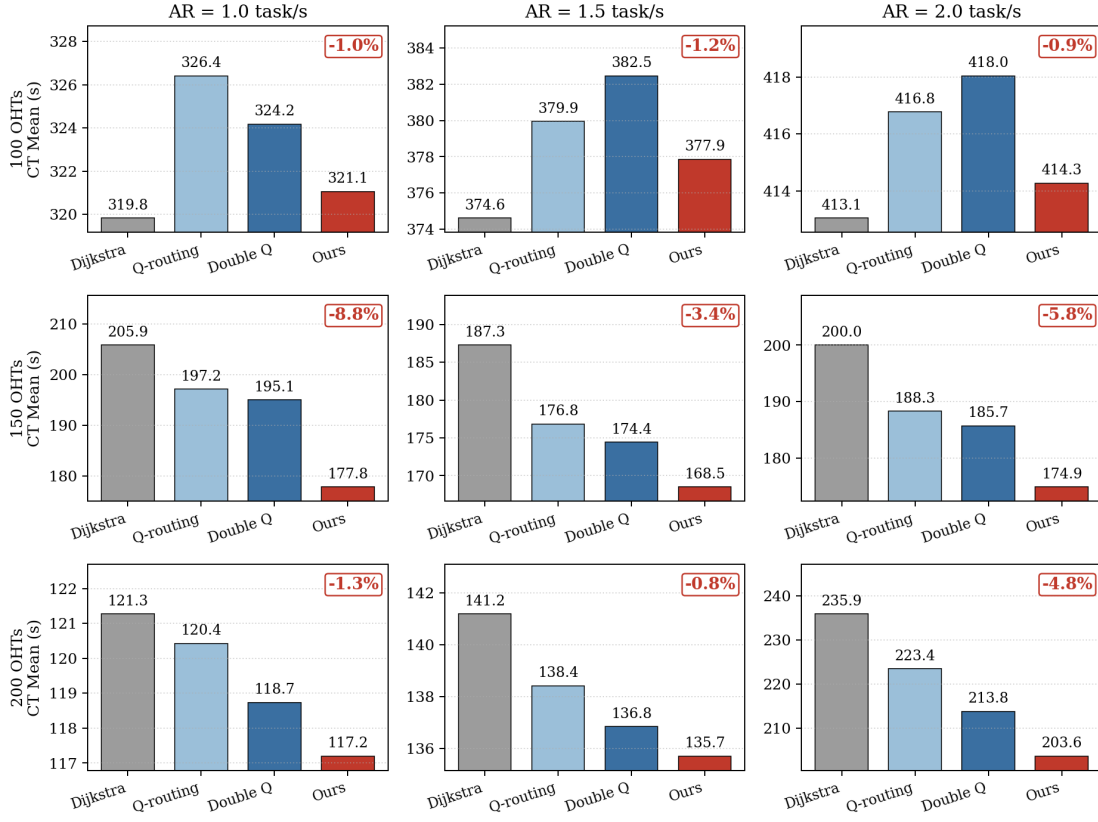
Fig. 6. CT Mean across the fleet-size and arrival-rate sweep, visualizing Table II. Red annotations report the relative change of QNeuralDouble from tabular Double Q-routing; negative values indicate lower CT Mean.
