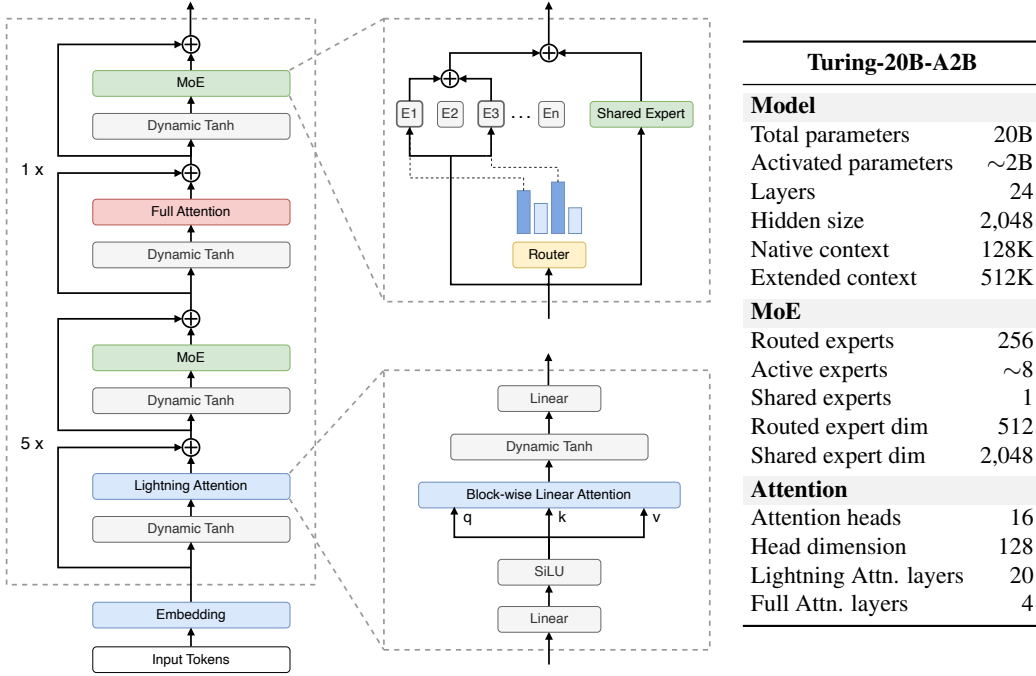
Figure 2: Overview of the Turing-20B-A2B architecture and model configuration. The decoder stack alternates groups of five Lightning Attention layers with one full-attention layer. The table summarizes the main architectural configurations.
