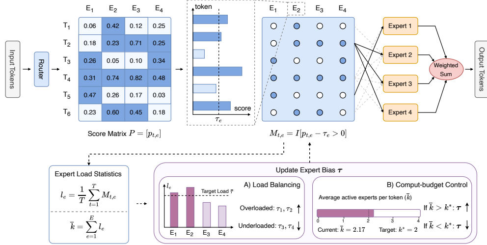
Figure 3: Overview of the routing strategy. Expert-specific thresholds determine token–expert assignments and are updated from expert-load statistics during training to track the target (1 - k^*/E) score quantiles. This unified quantile-tracking process naturally balances expert utilization, controls the average routing budget, and allows token-adaptive expert activation.
