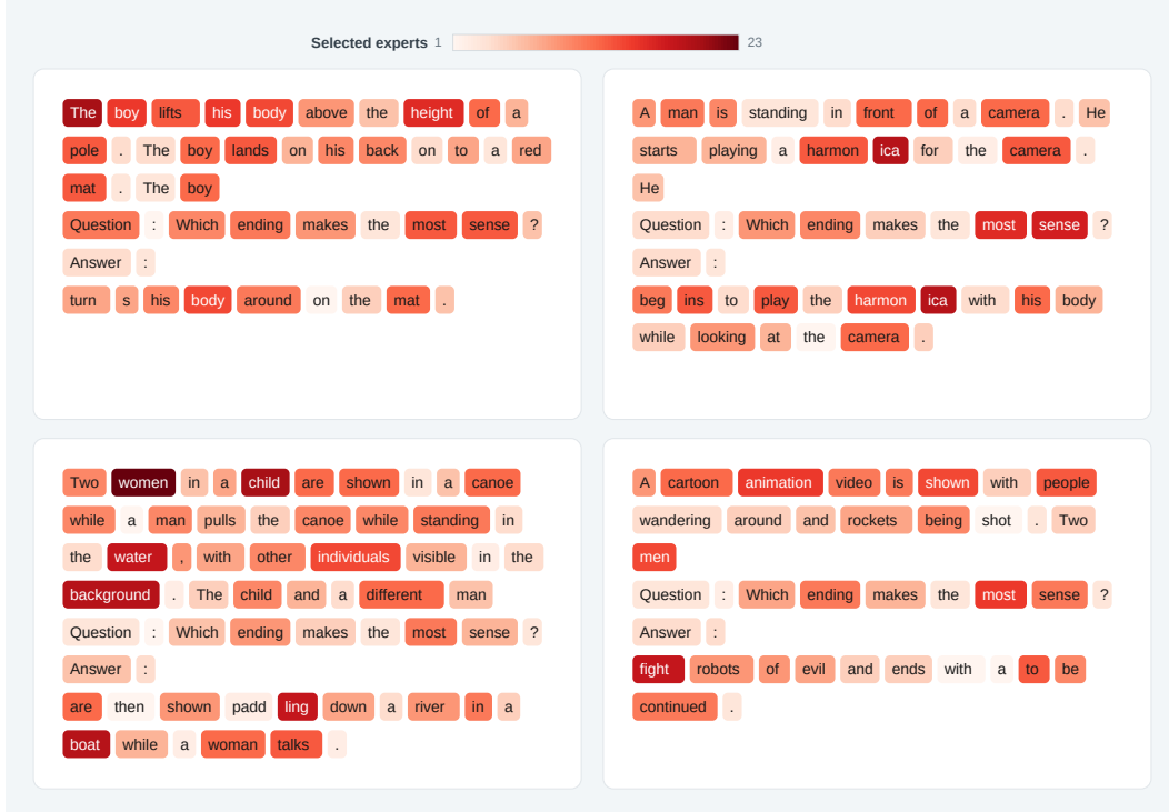
Figure 7: Token-wise expert allocation produced by Quantile Routing on representative HellaSwag examples. Darker tokens activate more routed experts. The expert count varies according to the contextual representation of each token, while maintaining an average routed-expert budget of eight. The always-active shared expert is excluded from the displayed counts.
