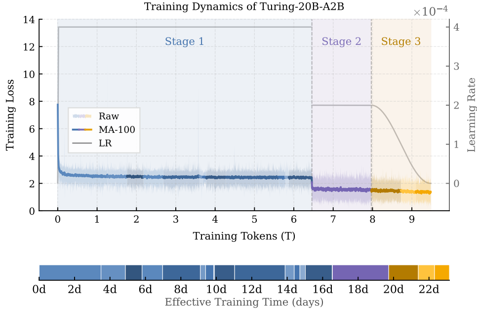
Figure 4: Training dynamics of Turing-20B-A2B over the three-stage main pretraining curriculum. The upper panel shows the raw training loss, its 100-step moving average (MA-100), and the learning-rate schedule over processed tokens, with dashed lines indicating stage boundaries. The lower timeline shows the effective training time of individual resumed runs.
