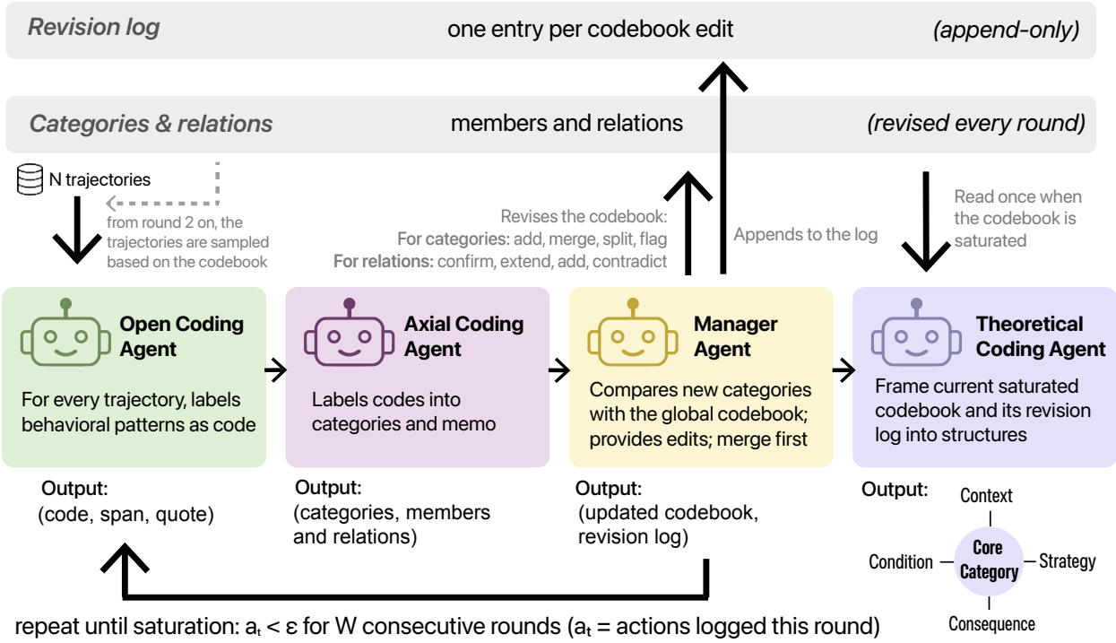
Figure 2 | Overview of our multi-agent qualitative coding pipeline.
