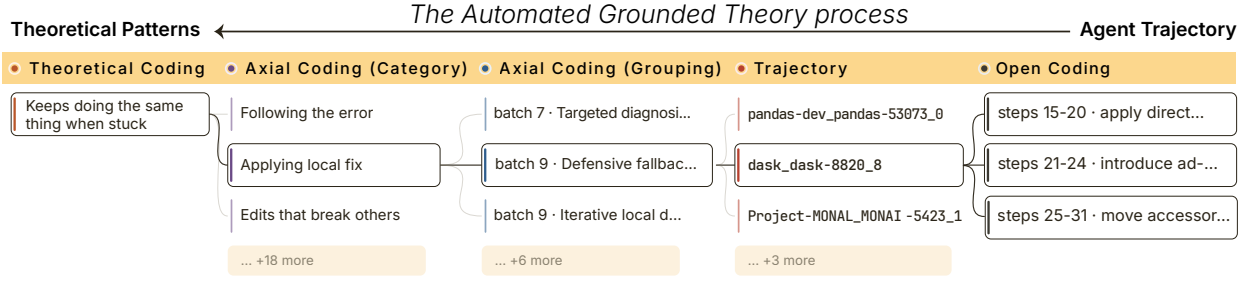
Figure 3 | An example of AutoTraceGT’s coding process. OpenCode annotates a raw trajectory with conceptual open codes; AxialCode groups open codes across batches into categories and typed relations; TheoreticalCode integrates the saturated codebook into a theoretical account. Every code, category, and claim points back to its supporting evidence, making each step auditable.
