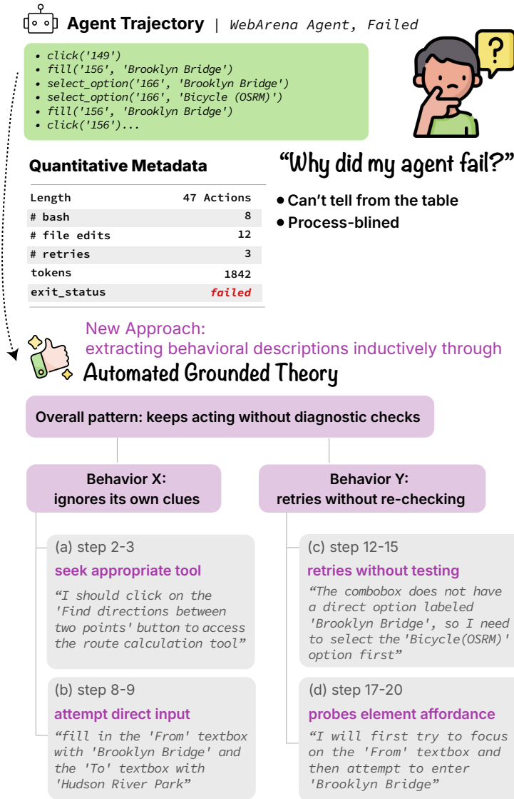
Figure 1 | Quantitative metadata records that an agent failed but is process-blind to why . Automated grounded theory (Glaser and Strauss, 1967; Saldaña, 2015) surfaces behavioral patterns from the agent’s own reasoning, e.g., keeps acting without diagnostic checks , decomposed into sub-behaviors ( ignores its own clues , retries without re-checking ) with step-level quoted evidence.
