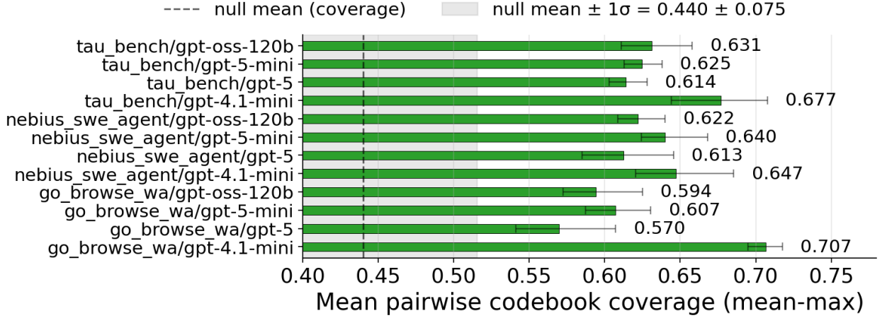
(a) Within-config replicate coverage vs. cross-config null
