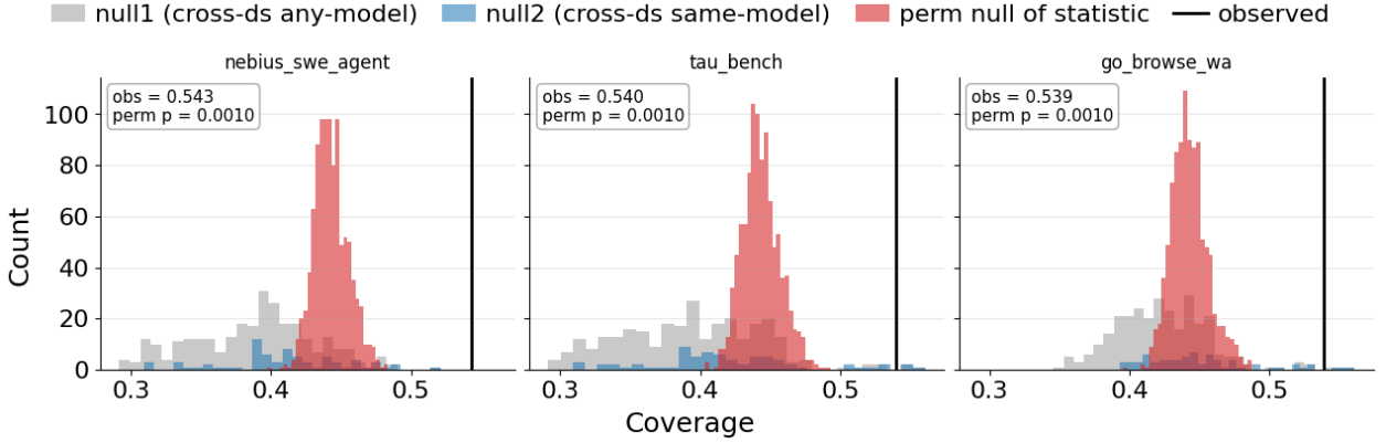
(b) Cross-LLM same-dataset coverage vs. null baselines
