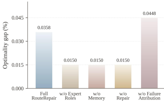
(a) TSP20
