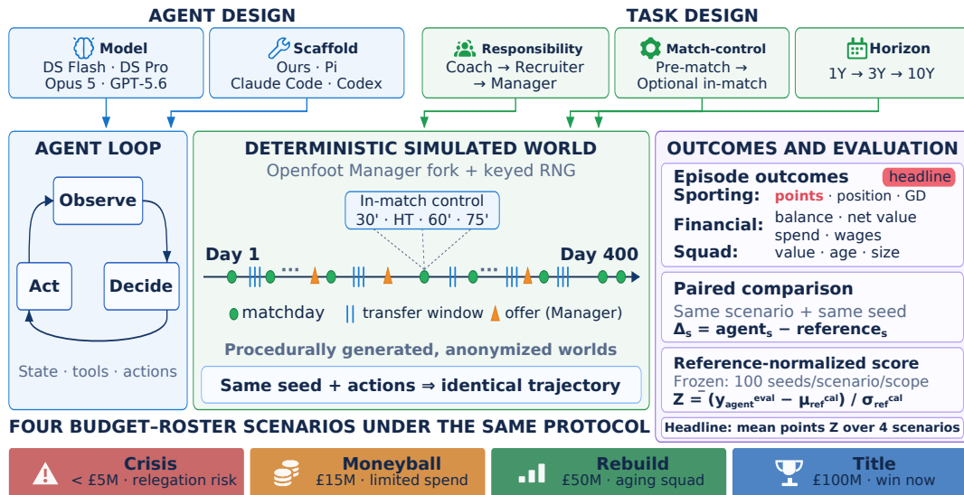
Figure 1: FromPitch2Board separates five experimental factors. Responsibility and horizon operationalize functional composition and temporal persistence; match-control granularity configures decision density, while model and scaffold support attribution under paired-seed evaluation.
