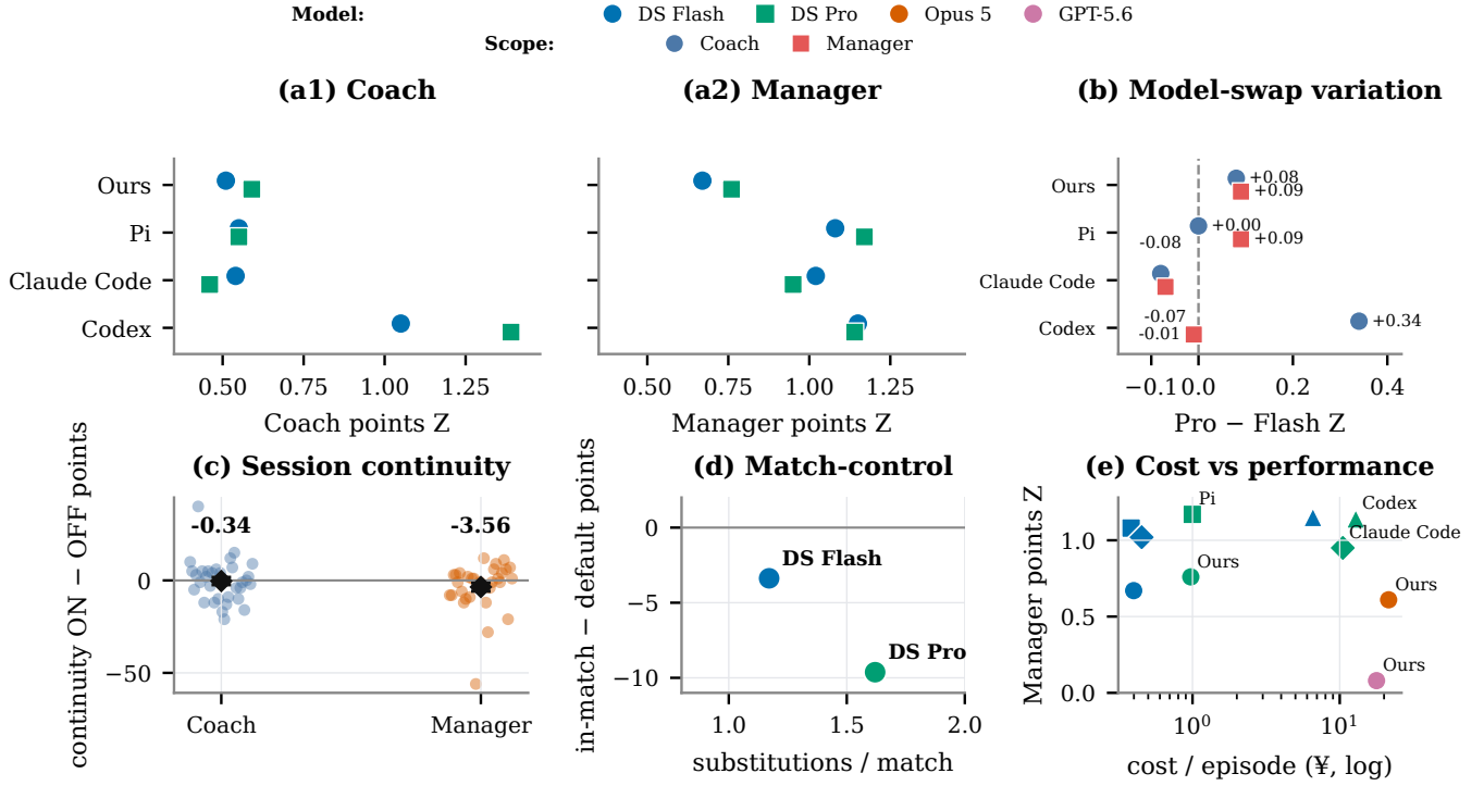
Figure 3: Scaffold and model contrasts within the Flash-Pro pair. Absolute scores and model swaps (a–b) precede continuity, match-control, and cost diagnostics (c–e); Manager scaffold spans are 0.48/0.41 Z versus a maximum Manager model swap of 0.09 Z.
