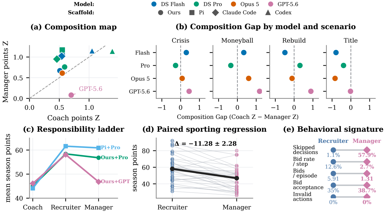
Figure 2: Responsibility expansion exposes a model-dependent behavioral signature. Panels connect the composition map and scenario gaps (a–b) to responsibility ladders, 32 paired GPT-5.6 episodes, and the resulting behavior (c–e).
