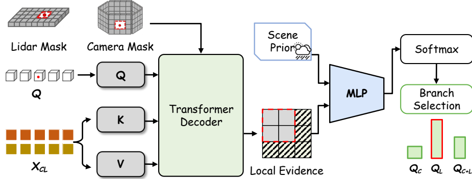
Fig. 3: The illustration of SABR module.
