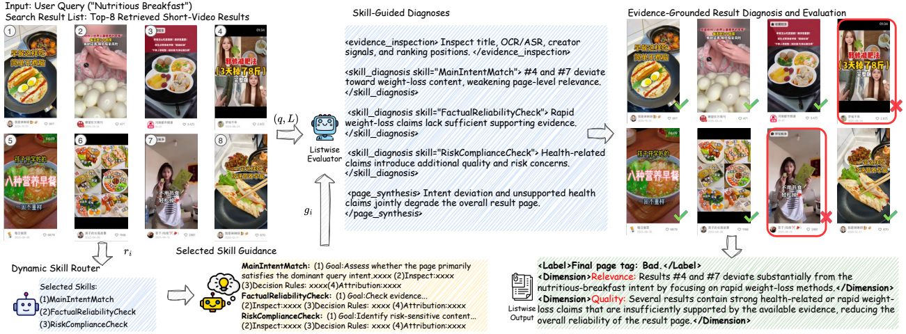
Figure 1: Illustrative example of skill-routed listwise evaluation in SEEK. The router selects task-relevant skills, and the listwise evaluator applies their guidance over the complete result page to produce a page-level judgment and attribution.
