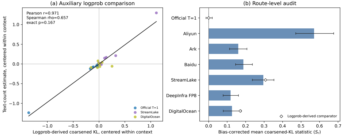
Figure 2 | Auxiliary consistency check for AFL. The left panel contains 36 context–route cells from three logprob-capable route conditions. Text-count AFL statistics and the logprob-derived coarsened-KL comparator show descriptive agreement after context centring; with only 3! = 6 route permutations, the exact route-level test is not confirmatory. The right panel shows the seven-route audit, in which the official control remains at the route-level null.
