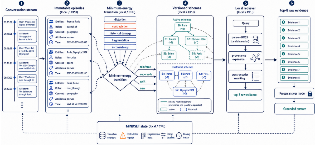
Figure 1: MINDSET stores immutable episodes, chooses minimum-energy transitions over versioned schemas, expands retrieved schemas back to provenance, and sends a bounded raw-evidence packet to the answer model.
