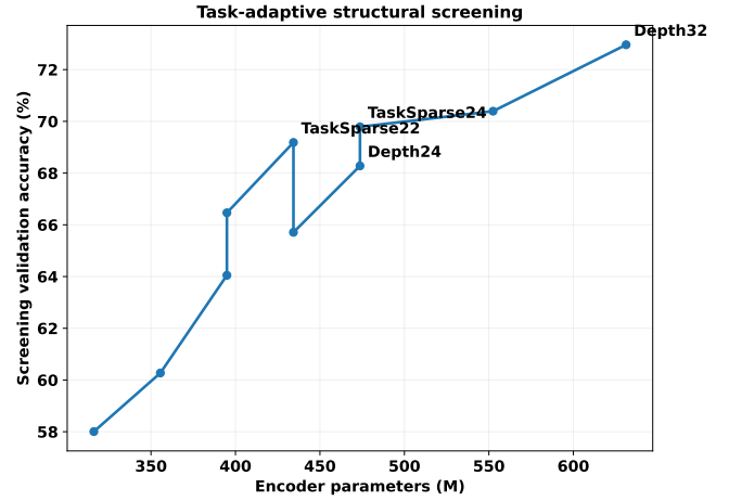
Figure 4: Validation-only structural screening of contiguous-depth and task-adaptive sparse candidates.
