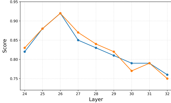
Figure 6: Probe performance across middle-to-late layers of Qwen3-14B.
