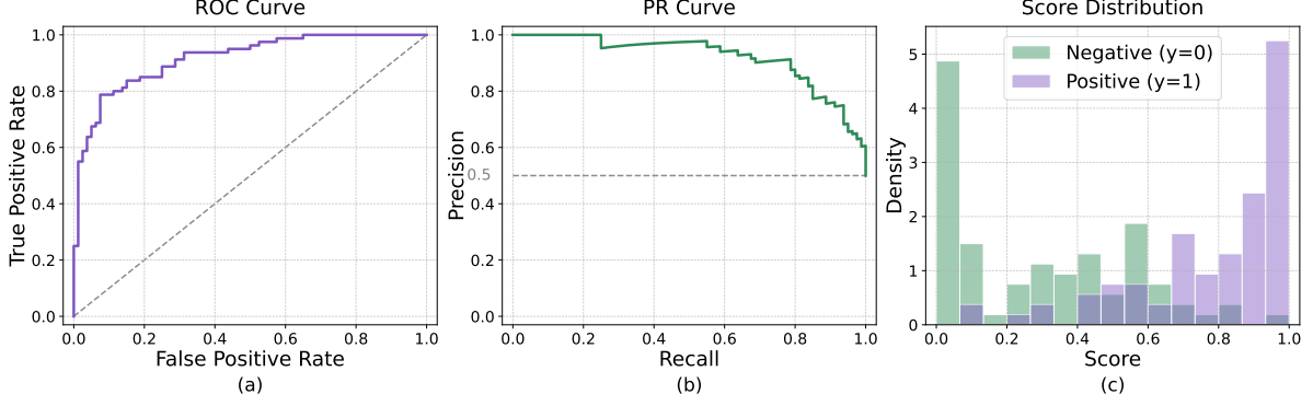
Figure 2: Probe results for late-stage pressure, including the ROC curve, PR curve, and probe score distributions. The results show that pressure-driven commits are linearly separable in hidden space.
