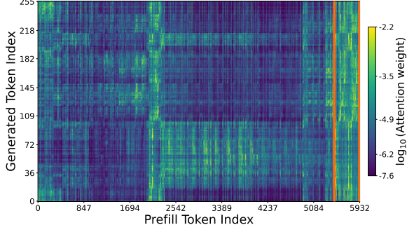
Figure 3: An attention example for a PresC node under the “+ Both” condition. The orange-marked region denotes the appended context.
