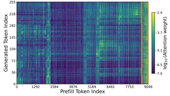
Figure 9: Attention heatmap showing that generated tokens attend to the appended context block under the “+ Both” condition.
