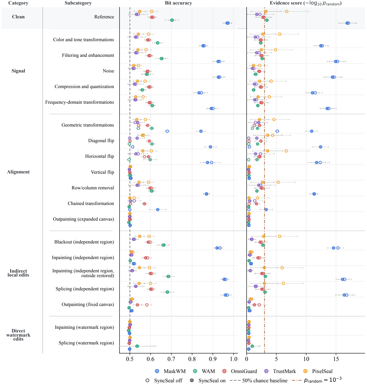
Figure 2: Payload recovery over the transformation taxonomy. Rows follow the transformation taxonomy in Appendix Table 3, with categories and subcategories shown at left. The left panel reports bit accuracy; the right panel reports the payload-length-aware evidence score, -\log_{10}(p_{\text{random}}) , where larger values indicate stronger evidence against random decoding after accounting for payload length. Open markers denote evaluation without SyncSeal and filled markers with SyncSeal; horizontal bars show the sample standard deviation across the four dataset means. The gray dashed line appears only in the bit-accuracy panel and marks the 50% chance baseline; the brown dash-dot line in the evidence-score panel marks the threshold p_{\text{random}} = 10^{-3} .
