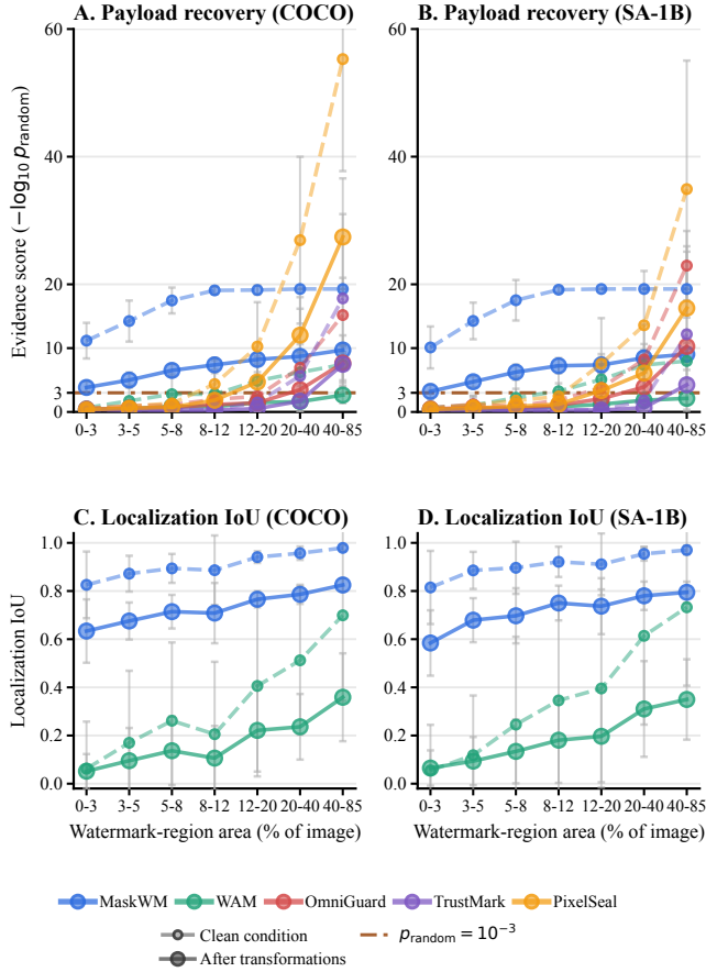
Figure 4: Larger watermark regions are associated with stronger payload recovery and watermark-region localization. The four panels group COCO and SA-1B examples by the fraction of image area covered by the watermark region, evaluated without SyncSeal. Panels A and B report the evidence score. Panels C and D report localization IoU for MaskWM and WAM. Dashed curves show clean-setting values. For the solid curves, bit accuracy and localization IoU are first averaged across all transformations for each image, and the evidence score is computed from the resulting mean bit accuracy. The brown dash-dot line in the payload-recovery panels marks p_{\text{random}} = 10^{-3} . Vertical bars show the sample standard deviation across image-level values within each area bin.
