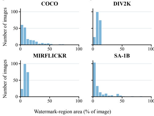
Figure 7: Watermark-region area by dataset. Distributions for clean MaskWM examples without SyncSeal. COCO and SA-1B use native masks; DIV2K and MIRFLICKR use sampled masks. Mean areas are 15.22% (COCO), 12.50% (SA-1B), and 8.80% (DIV2K and MIRFLICKR).
