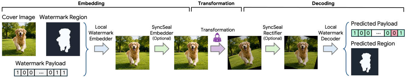
Figure 1: Evaluation pipeline. (i) Embedding . Given a cover image, a watermark mask, and a binary payload, the watermarking method embeds the payload within the masked region. When SyncSeal is enabled, its embedder then adds a synchronization signal across the image. (ii) Transformation . The resulting image undergoes one of the 55 benchmark transformations. (iii) Decoding . When SyncSeal is enabled, its rectifier first attempts to restore the coordinate frame expected by the watermark decoder; otherwise, both SyncSeal operations are skipped. The watermark decoder then recovers the payload and, when supported, localizes the watermarked region. For runs with and without SyncSeal, we report payload recovery for all methods, pixel-level localization for MaskWM and WAM, and also image fidelity in the clean setting.
