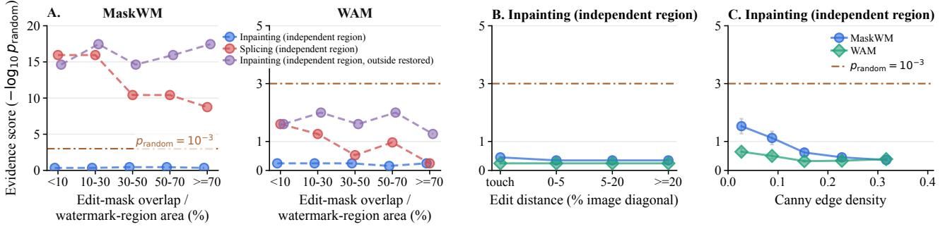
Figure 5: Payload recovery under local edits. The panels examine three factors in local edits: edit-mask overlap, distance from the watermark region, and edge density within preserved watermark-region pixels. Panel A compares inpainting (independent region), splicing (independent region), and the inpainting (independent region, outside restored) control for MaskWM (left) and WAM (right). Panel B shows that increasing the edit-to-watermark distance for inpainting (independent region) does not restore recovery. Panel C divides inpainting (independent region) examples with less than 5% edit-mask overlap into quintiles by Canny edge density over watermark-region pixels outside the edit mask. Markers show the mean edge density and evidence score in each quintile, and vertical bars show standard errors of the evidence-score means across examples within that quintile. MaskWM has higher evidence scores when those preserved pixels have lower Canny edge density, while WAM’s evidence scores remain close to zero. Brown dash-dot lines mark the evidence-score threshold p_{\text{random}} = 10^{-3} .
