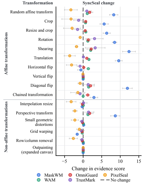
Figure 6: SyncSeal effect on payload recovery under changes in alignment. Rows include only transformations in the alignment category, grouped into affine and non-affine blocks. Points report the change in payload-length-aware evidence score, -\log_{10} (p_{\text{random}}) , from enabling SyncSeal; positive values indicate stronger payload recovery with SyncSeal. Horizontal bars show the sample standard deviation across the four dataset-level changes.
