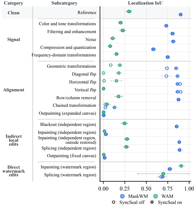
Figure 3: Localization accuracy over the transformation taxonomy. Rows follow the transformation taxonomy in Appendix Table 3. The plot reports localization IoU for MaskWM and WAM, the methods that return directly comparable pixel-level maps of watermark presence. Open markers denote SyncSeal off and filled markers denote SyncSeal on; horizontal bars show the sample standard deviation across the four dataset means.
