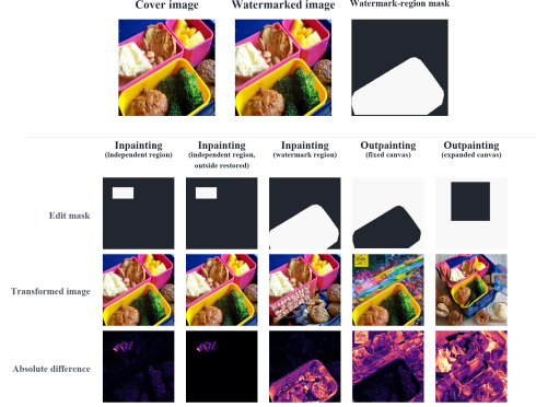
Figure 8: Inpainting and outpainting protocols. Examples show edit masks, transformed images, and absolute differences. The outside-restored control restores pixels outside the edit mask; fixed-canvas outpainting regenerates surrounding content, whereas expanded-canvas outpainting extends and rescales the canvas.
