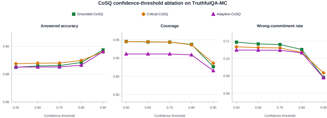
Figure 3: Confidence-threshold ablation for the three CoSQ variants on TruthfulQA-MC. Panels report answered accuracy, coverage, and unconditional wrong-commitment rate. Colors and marker shapes distinguish the variants; all horizontal axes show \tau from 0.50 to 0.90.
