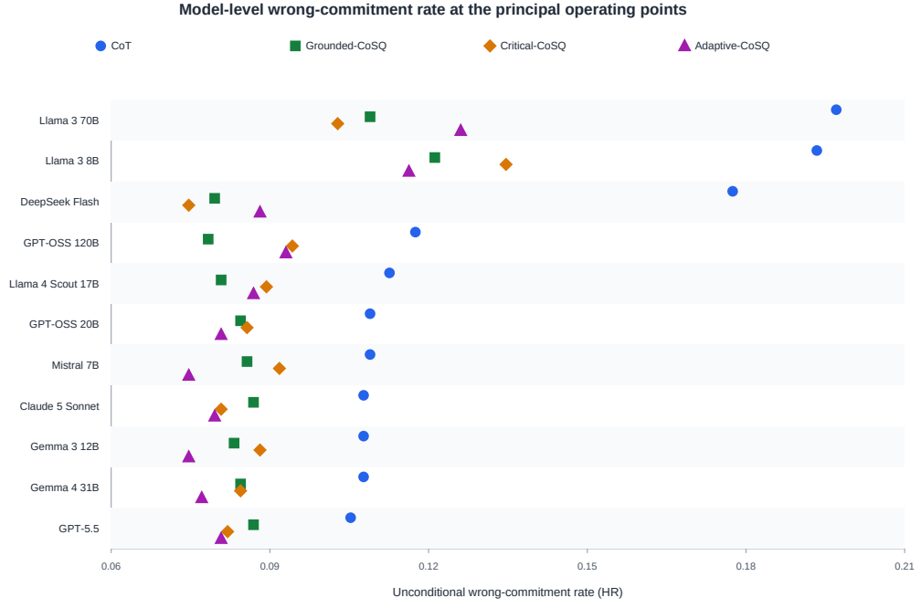
Figure 5: Model-level unconditional wrong-commitment rate for CoT and the three \tau = 0.90 CoSQ variants. Lower values are better. Colors and marker shapes have the same meaning as in Figures 2–3.
