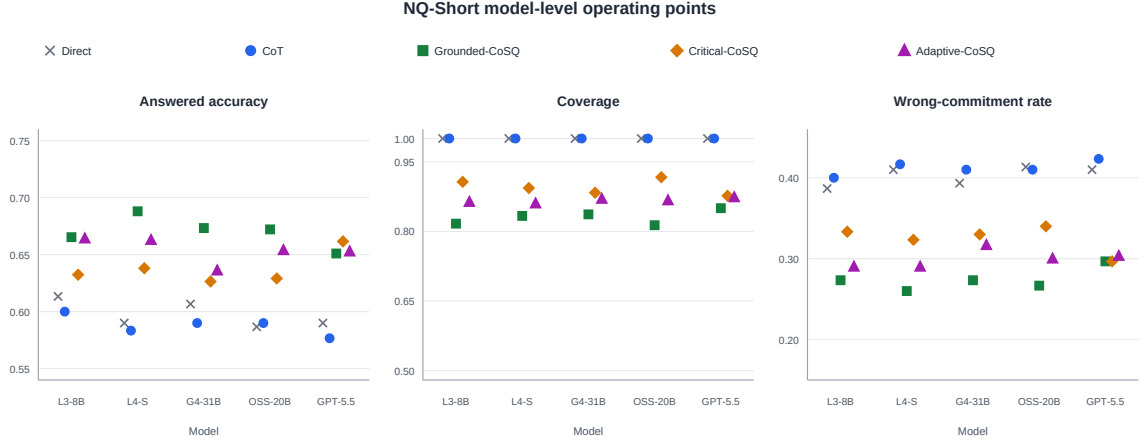
Figure 4: Model-level NQ-Short results for the five-model secondary panel. Each panel reports one metric; colors identify the five evaluation conditions. The figure is descriptive and is not pooled with the primary TruthfulQA-MC analysis.
