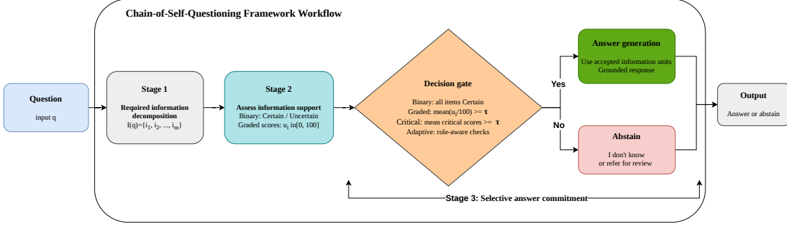
Figure 1: Chain-of-Self-Questioning. The model identifies required information, evaluates its support, applies a confidence gate, and either abstains or generates an answer using accepted information units.
