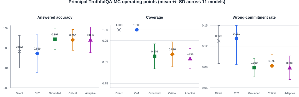
Figure 2: Principal TruthfulQA-MC outcomes across the eleven-model panel. Points show model-macro means and error bars show one standard deviation. Colors and marker shapes identify Direct, CoT, and the three CoSQ variants consistently across figures.
