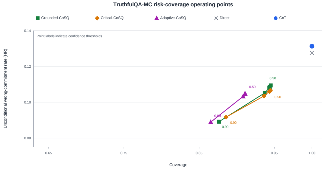
Figure 7: TruthfulQA-MC wrong-commitment–coverage operating points. Connected markers show each CoSQ family from \tau = 0.50 to 0.90 ; isolated markers show the forced Direct and CoT baselines. Coverage is reported as a tunable operating characteristic rather than an error measure.
