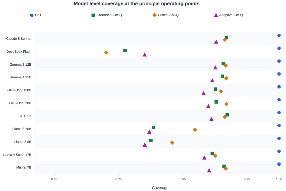
Figure 6: Model-level coverage for CoT and the three \tau = 0.90 CoSQ variants. Coverage is an operating characteristic: lower values indicate that more questions are explicitly referred rather than answered.
