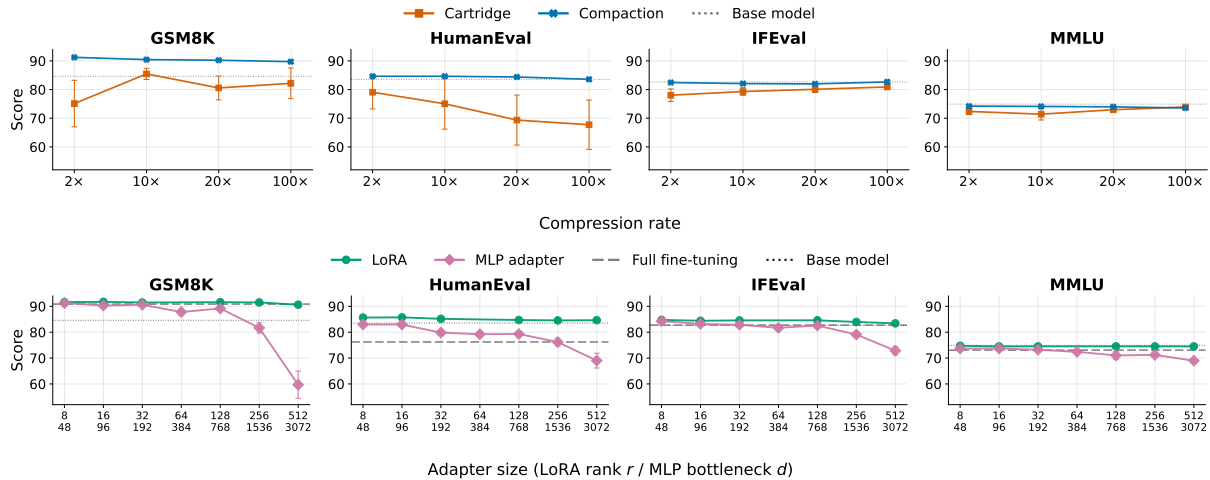
Figure 3: Forgetting on control benchmarks (Qwen3-8B). The score is averaged across the five source datasets, and error bars are the standard error across those datasets. (Top) The representation-based methods are swept over compression rate; the lowest-compression column merges the 2\times and 3\times points (the two longest datasets use 3\times ). (Bottom) The parametric methods are swept over adapter size.
