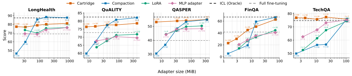
Figure 1: Single-document score versus adapter size (MiB, log scale). Cartridges and Compaction are swept over compression rates 2\times , 10\times , 20\times , 50\times , and 100\times . LoRA and the MLP adapter use the rank and bottleneck dimension that match the KV-cache memory footprint at each rate.
