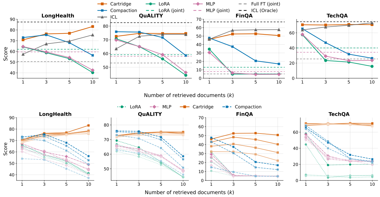
Figure 2: Multi-document results (Qwen3-8B). Score versus the number of retrieved documents k , composing the top- k retrieved per-document artifacts. (Top) Fixed adapter size. ICL refers to RAG in this setting, ICL (Oracle) is the in-context upper bound with the gold document in context, and Joint is a single adapter trained on all documents. (Bottom) Varying adapter size. Each method is swept over the storage-matched compression ratios (where available), with method encoded by color and compression rate by shade (dark = larger adapter / lower compression).
