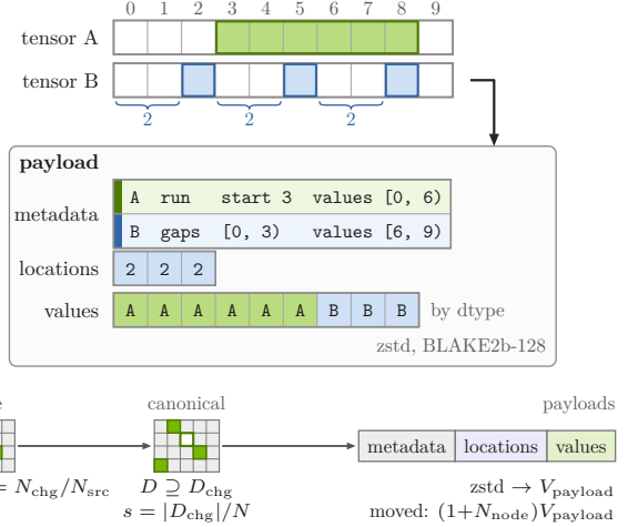
Figure D.3 | Top: payload format. To decode gaps, start at -1 and add each gap plus one: gaps 2, 2, 2 yield positions 2, 5, 8. Values have the width of their tensor’s dtype. Bottom: quantities behind payload volume. Owners find N_{\text{chg}} changes among N_{\text{src}} source elements, which gives the element change rate s_{\text{src}} . The emitted destinations D contain the changed destinations D_{\text{chg}} , whose share of the N canonical elements is the canonical change density s . When a mapping is not a representation-preserving bijection, D can also hold an unchanged destination, drawn outlined. Payloads carry metadata, locations, and values, and with N_{\text{node}} rollout nodes, object storage moves about (1+N_{\text{node}})V_{\text{payload}} per attempt in uploads and downloads.
