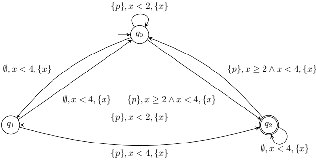
Fig. 1. The simple timed automaton used in Section VI-A. Note that the alphabet size is 2.
