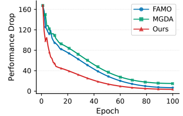
(b) CityScapes
