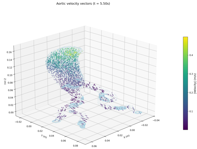
Figure 8: Representation of internal velocity vectors at random domain points for t = 5.5 s (systole)
