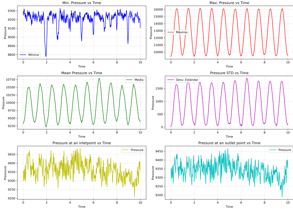
Figure 9: Temporal evolution of the pressure: minimum (top left), maximum (top right), mean (center left), standard deviation (center right), pressure at an inlet point (bottom left), and pressure at an outlet point (bottom right).
