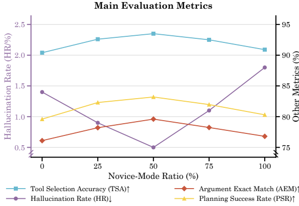
Figure 5: Clarification ratio ablation. PSR, TSA, AEM (right y axis), and Hal.Rate (left y axis) across five novice fractions from 0% to 100%.
