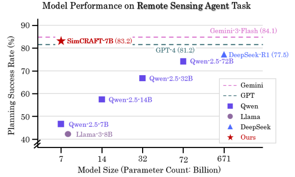
Figure 1: Performance vs. model size. SimCRAFT-Qwen2.5-7B (red star) compared with open-weights and closed-source baselines.
