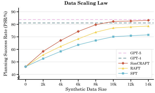
Figure 6: Data scaling law. PSR vs. SimRS-14k corpus size, with GPT-4 / GPT-5 zero-shot reference lines.
