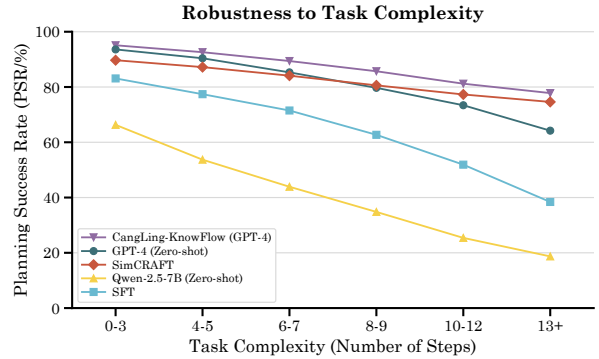
Figure 7: Long-horizon robustness. PSR by trajectory-length bucket.
