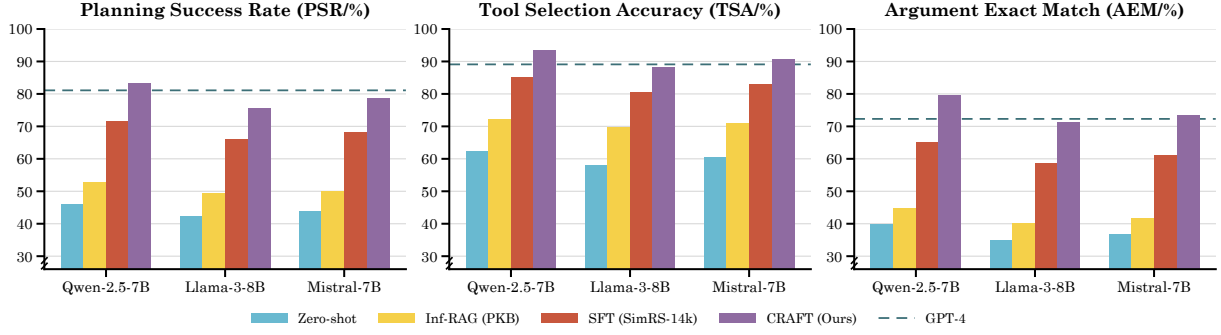
Figure 4: Joint backbone × training-paradigm ablation. Three 7B-scale backbones each evaluated under four paradigms (Zero-Shot, Inf-RAG, vanilla SFT, CRAFT).
