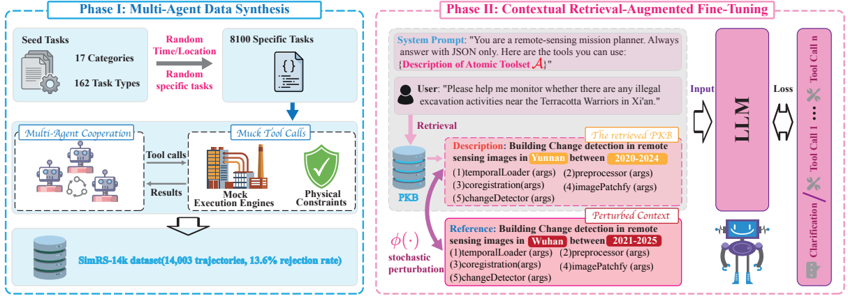
Figure 2: Overview of the SimCRAFT framework. Phase I expands 162 seed tasks into the SimRS-14k corpus; Phase II distills procedural knowledge into a 7B backbone via Contextual Retrieval-Augmented Fine-Tuning.
