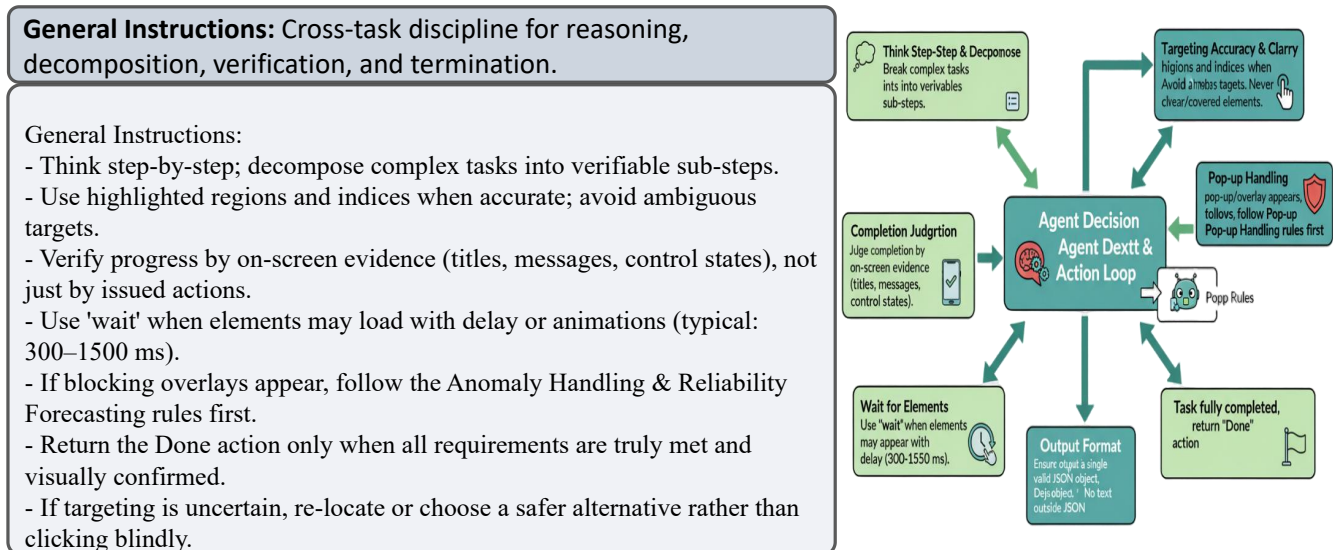
Figure 16: General instruction template. Defines structured reasoning, precise targeting, verification, controlled waiting, and disciplined termination to ensure robust, evidence-driven task execution.
