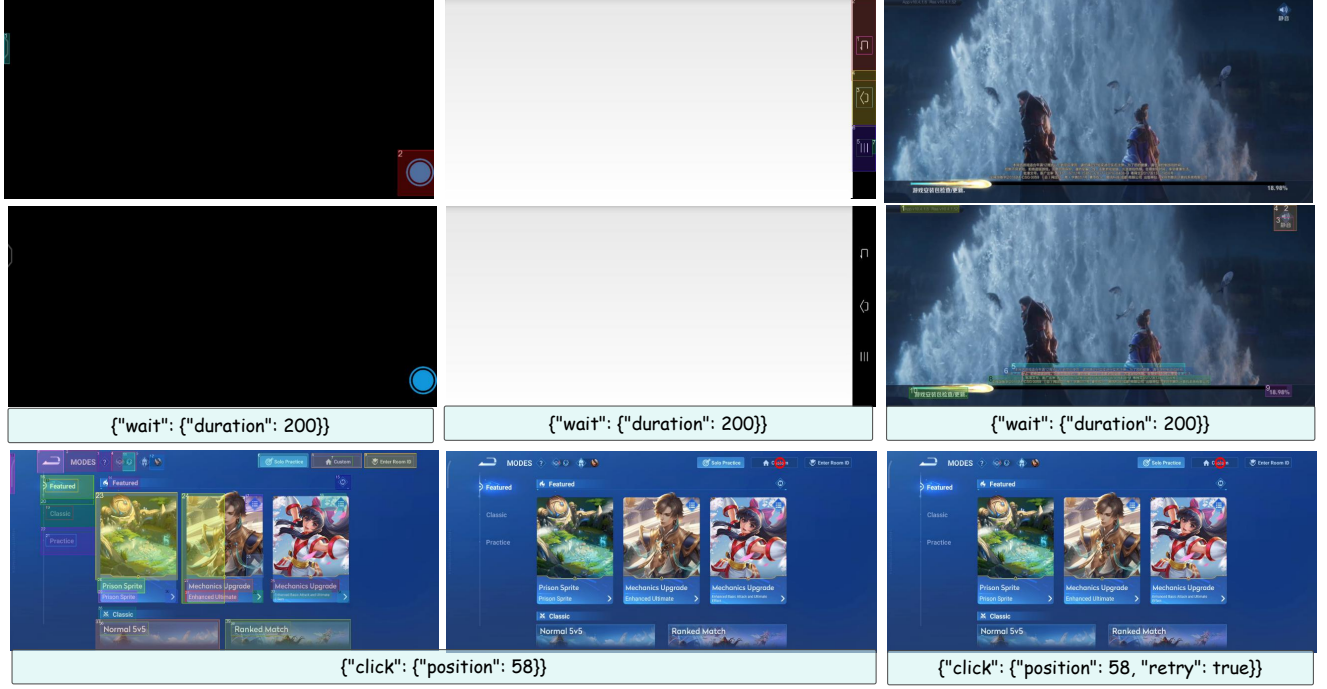
Figure 19: Environment disturbances. A lightweight routine—short waits plus index prioritized safe retries stabilizes black/white screens, delayed loads, and network stalls; the figure shows concrete wait and retry commands for representative cases.
