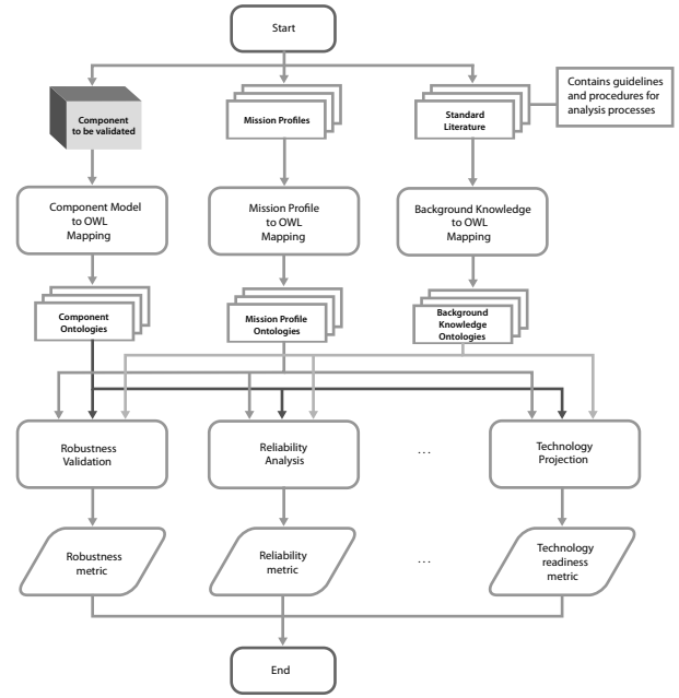
Fig. 8: General process flow
