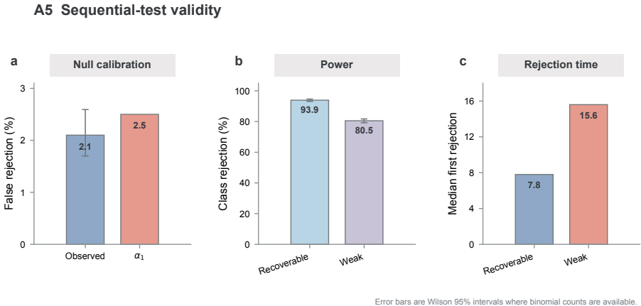
Figure 10: Sequential-test validity. The observed false-rejection rate is 2.1% under the sufficient-class null versus the stage-1 allocation \alpha_1 = 2.5\% . Class-rejection power is 93.9% on recoverable misspecification and 80.5% on weakly distinguishable misspecification, with median first rejection at 7.8 and 15.6 experiments.
