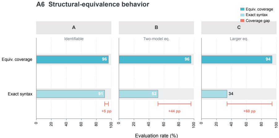
Figure 11: Structural equivalence. Exact syntax recovery falls as the observational equivalence class grows, while coverage of a valid equivalent mechanism remains 96%, 96%, and 94% for identifiable, two-model-equivalent, and larger-equivalence tasks.
