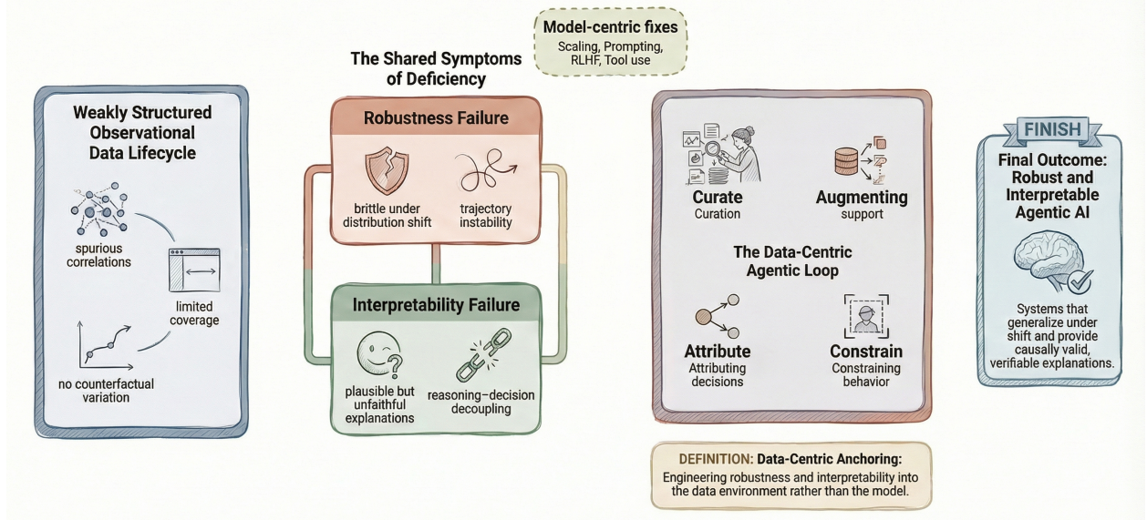
Figure 1: Robustness and interpretability failures in agentic AI are not isolated issues, but co-symptoms of a shared structural deficiency in the data lifecycle. Weakly structured observational data lacks the variation needed to support invariant learning and counterfactual validation, motivating a data-centric anchoring perspective.
