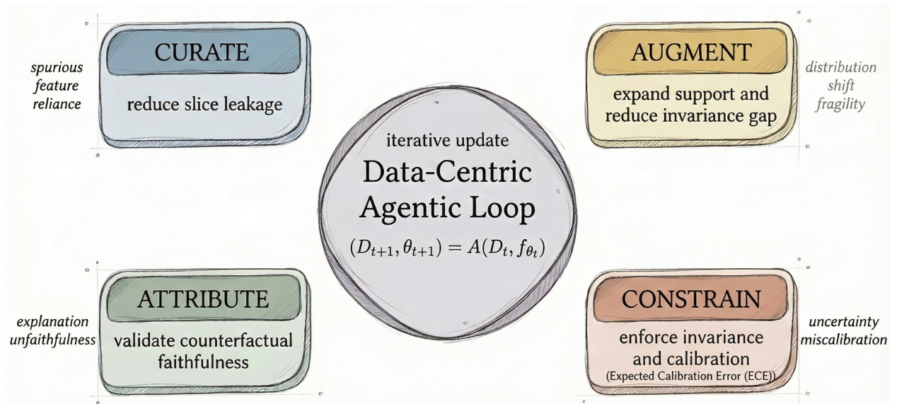
Figure 2: The Data-Centric Agentic Loop iteratively refines both the dataset and the agent through four coupled stages: Curate, Augment, Constrain, and Attribute. Each stage addresses a distinct failure signal and produces the conditions required for the next, forming a failure-driven closed loop for robust and interpretable agentic AI.
