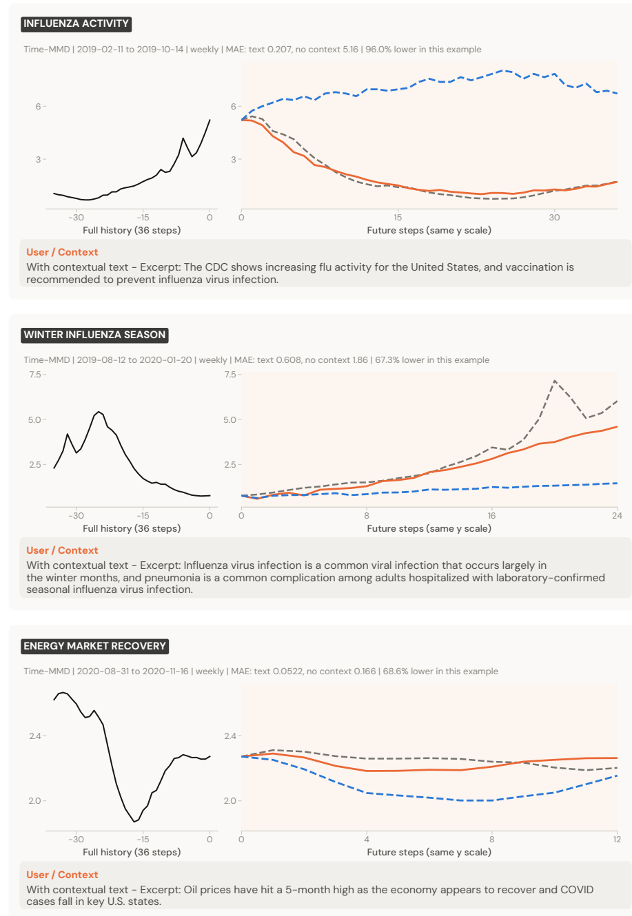
Figure 13. Selected Time-MMD test forecasts with matched contextual-text ablations. Orange uses the full dataset-provided textual context; dashed blue removes that context while retaining the same forecast instruction, numerical history, and horizon. Dashed gray is the observed future. Text below each panel is a verbatim excerpt of the full context used for prediction. MAE is measured over the complete future horizon in source units; reductions describe these selected examples.
