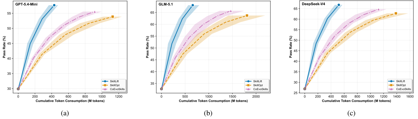
Figure 3: Token consumption vs. average pass rate on SkillsBench across three backbone models. Curves are smoothed up to the 0.9 quantile and truncated when no improvement is observed for two consecutive rounds. SkillLift reaches higher pass rates at substantially lower token cost than SkillOpt and CoEvoSkills.
