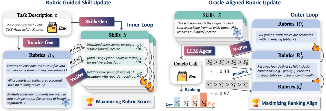
Figure 2: Overview of SKILLIFT. The system alternates between two phases: inner loop (rubric-guided skill update) where the rubric R scores and guides skill revision without oracle rollouts, and outer loop (oracle-aligned rubric update) where oracle evaluations on frozen skills re-align R via Kendall’s \tau .
