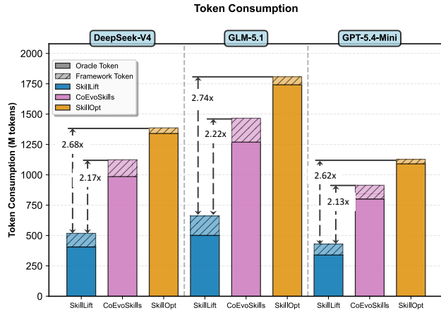
Figure 4: Average token cost to first reach the 0.9 quantile of total pass-rate score on SkillsBench. SkillLift reduces token overhead by 40–70% compared to baselines.
