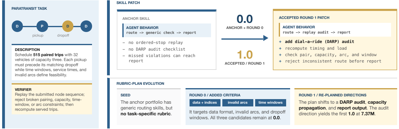
Figure 6: Case study on a SkillsBench paratransit scheduling task, showing rubric and skill co-evolution across two outer rounds.
