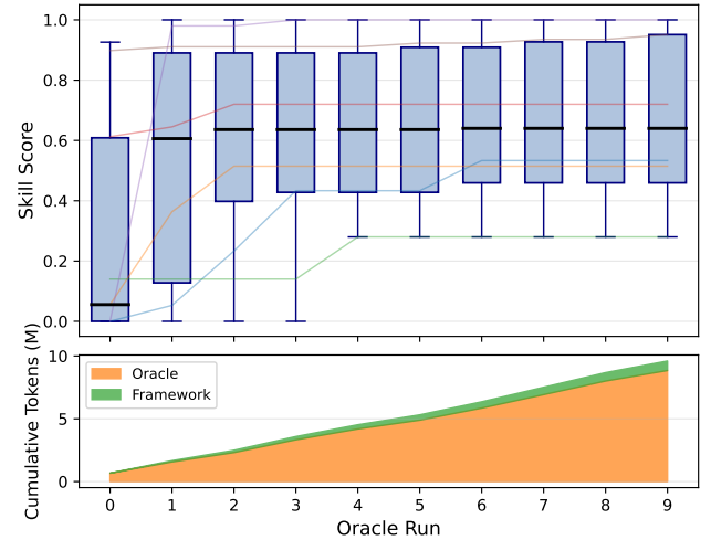
Figure 1: Pilot study (10 WildClawBench (Ding et al. 2026) tasks, 10 rounds, 3 seeds). Top: per-round averaged best/mean/worst skill scores. Bottom: averaged cumulative oracle vs. framework tokens. Scores show high variance and poor scaling; oracle cost dominates and grows.
