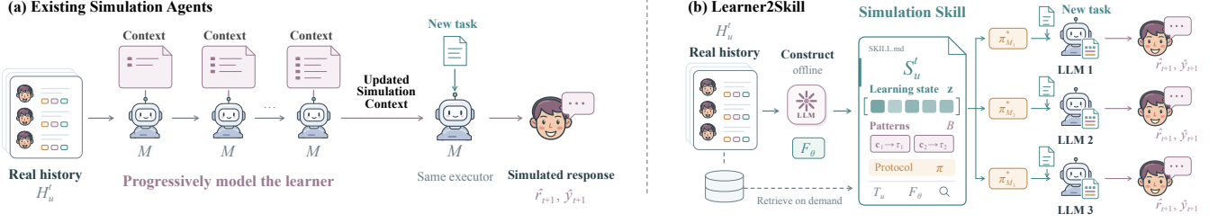
Figure 1: Comparison of (a) existing LLM simulation agents that progressively model learners from interaction histories, and (b) Learner2Skill, which constructs reusable Simulation Skills for cross-executor simulation and online evolution.
