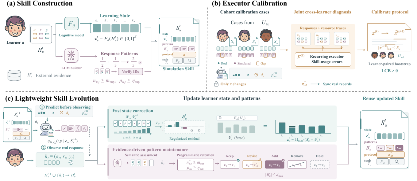
Figure 2: Overview of Learner2Skill. (a) Construct learner-specific Skills from real histories. (b) Calibrate a shared execution protocol through cross-learner diagnosis and held-out validation. (c) Update learner states and response patterns from new real interactions, with model parameters and the calibrated protocol fixed.
