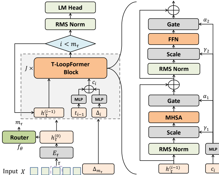
Figure 1: The architecture of T-LoopFormer, which could achieve token-level elastic-depth through a dynamic token-choice router.
