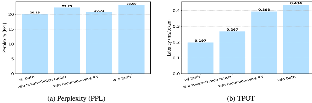
Figure 3: The influence of token-choice router and recursion-wise KV cache. Tested on FineWeb-Edu-100B validation set and at 24x FLOPs, w/: with, w/o: without. (a): perplexity results and (b): time per output token results.
