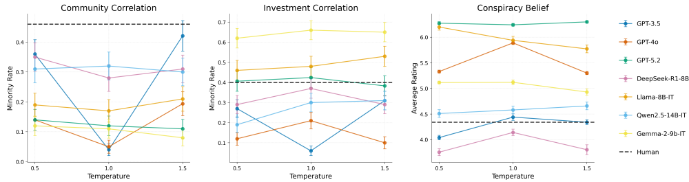
Figure 11: Human and LLM responses on three tasks across varying temperatures T .
