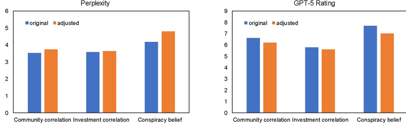
Figure 15: Perplexity and rating by GPT-5 for original and adjusted responses.
