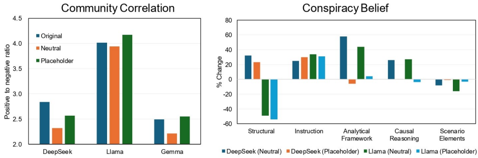
Figure 14: Mean-pooling SAE feature-shift analysis under placeholder reminder. Left: ratio of activation scores for positive and negative behaviors in the community correlation task. Right: percentage change in pooled activation score for each feature category in the conspiracy belief task.
