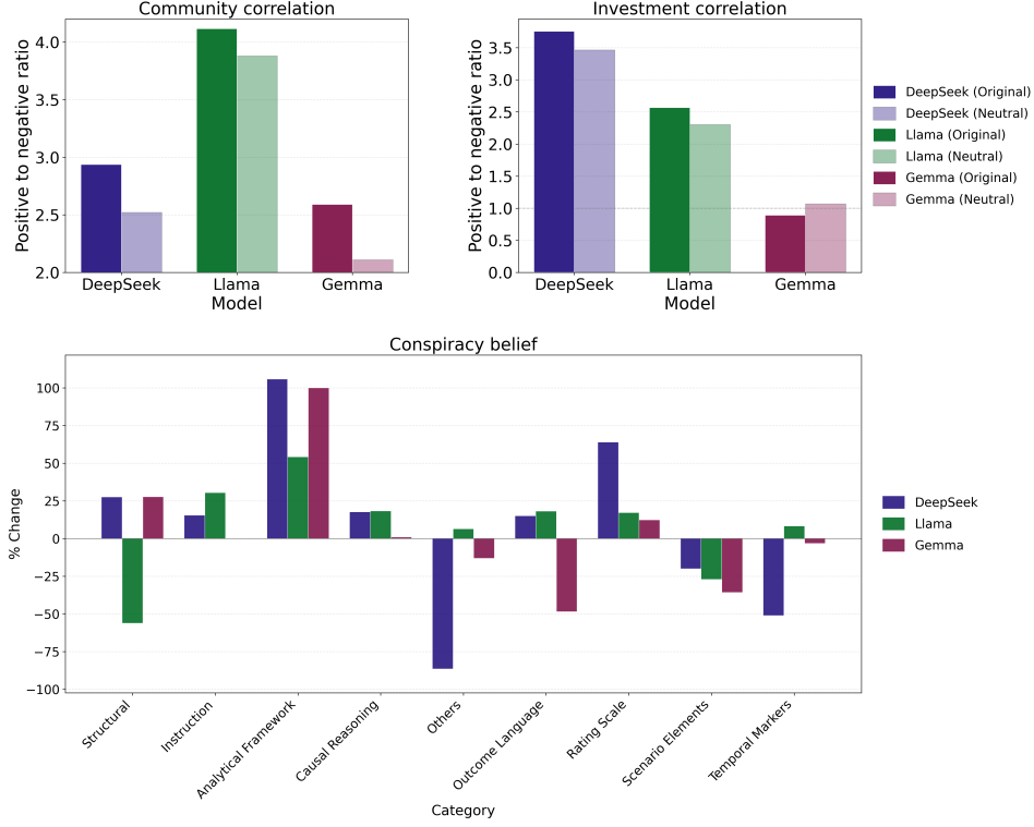
Figure 13: Mean-pooling SAE feature-shift analysis. Upper: ratio of activation scores for positive and negative behaviors in the community and investment correlation tasks. Bottom: percentage change in pooled activation score for each feature category from original to correlation-neutral samples in the conspiracy belief task.
