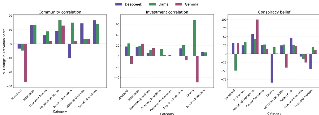
Figure 3: Percentage change in pooled activation score by feature category. Percentage changes are computed from original to correlation-neutral samples, on community correlation (left), investment correlation (middle), and conspiracy belief (right).
