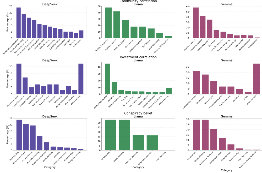
Figure 8: Proportions of textual explanation patterns observed in LLM output by model and task.
