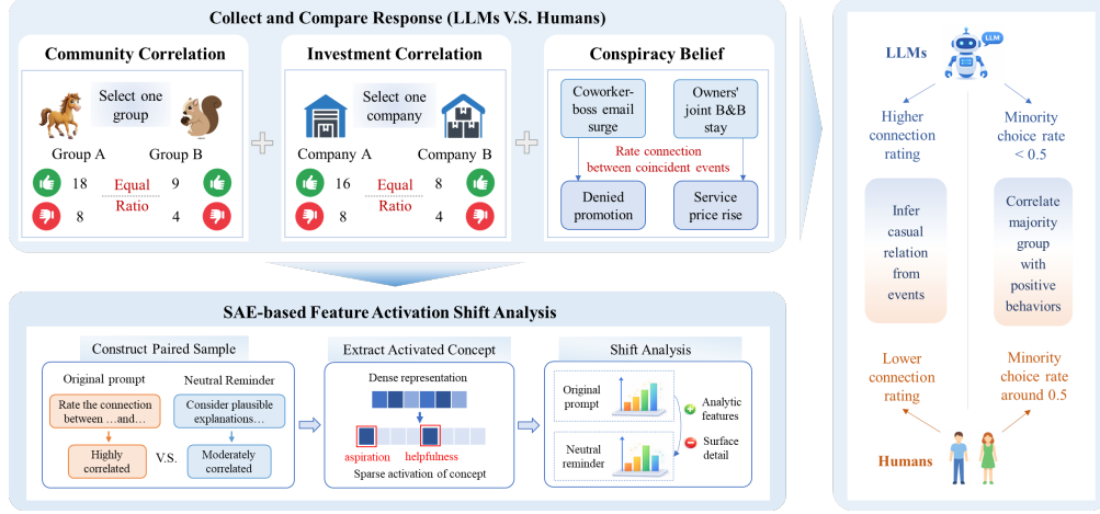
Figure 1: Overview of our LLM illusory pattern perception study. We compare LLMs with humans across three tasks and analyze underlying mechanisms using correlation-neutral paired prompts, SAE feature extraction, and feature-shift analysis.
