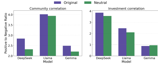
Figure 10: Ratio of activation scores for positive and negative behaviors in the community (left) and investment (right) correlation tasks.
