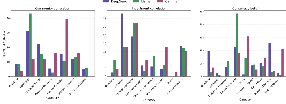
Figure 9: Percentage of activation score for each category for original prompt by model and task. Percentage of activation score for each category for original prompt by model and task.
