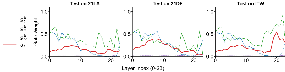
Figure 5: Analysis of learned gating distributions on different sets. The plot displays the distributions of component gates and the final aggregated importance coefficient (red solid line). The distinct activation patterns across different datasets confirm that the HAG module dynamically reconfigures its attention to capture domain-specific forensic traces while suppressing irrelevant signals.
