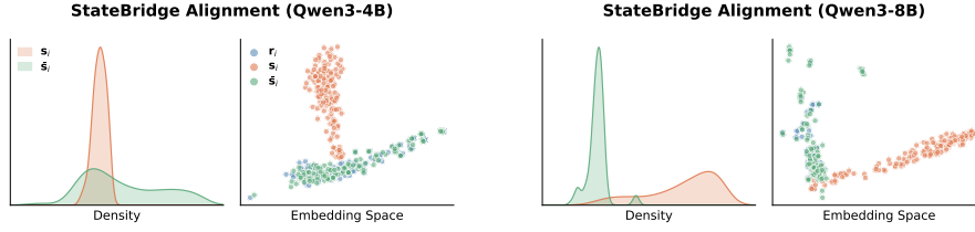
Figure 3: Principal component analysis (PCA) density (left) and PCA scatter of the embedding space (right) for Qwen3-4B and Qwen3-8B. Orange: message hidden states s_i ; blue: reference embeddings r_i ; green: aligned prefix \tilde{s}_i .
