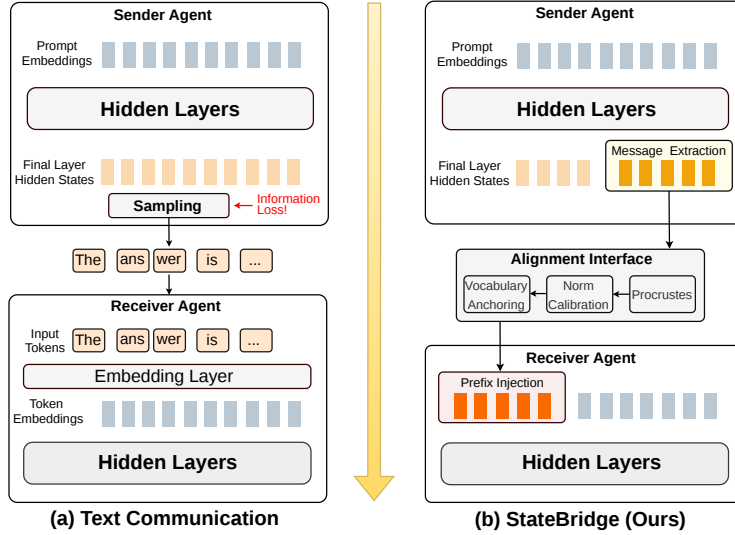
Figure 1: Overview of StateBridge. Standard text communication (a) transforms the sender’s message to discrete token identities via sampling, which causes information loss, whereas StateBridge (b) extracts message hidden states from the sender, aligns them with the input embedding space, and prepends the resulting prefix to the receiver’s prompt.
