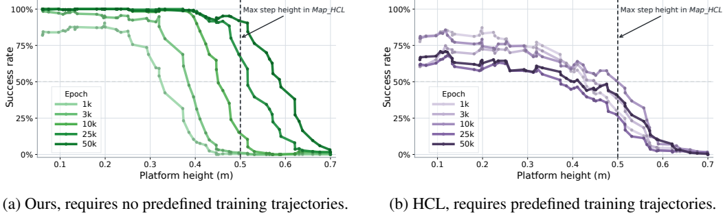
Figure 6: Platform-climbing evaluation across approach directions. Each value is the average success rate over diverse approach directions, where our method shows more robust traversal than HCL.
