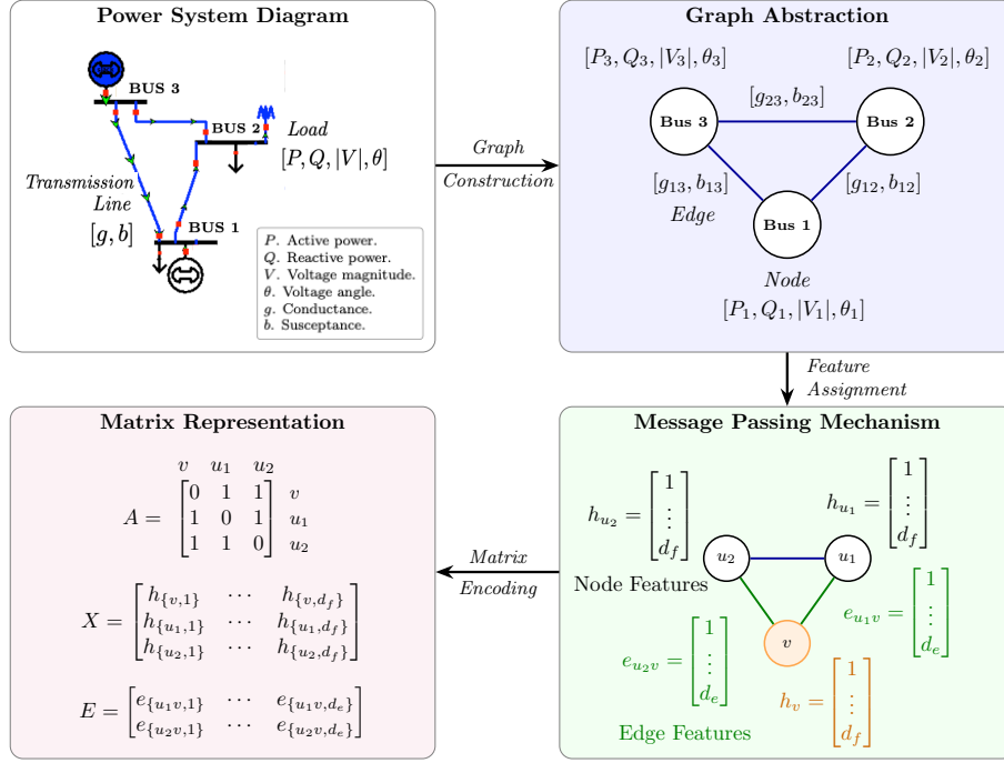
Fig. 1. Transition from a physical power grid to its graph-based representation for GNNs. (top-left) A three-bus system with node features (P, Q, |V|, \theta) and edge features (g, b) . (top-right) Graph abstraction mapping buses to nodes and transmission lines to edges while preserving features. (bottom-right) Message passing at node v , aggregating information from neighbors u_1 and u_2 using node and edge features; u and v denote neighboring nodes, d_f is the node-feature dimension, and d_e is the edge-feature dimension. (bottom-left) Matrix representation with adjacency matrix A , node-feature matrix X \in \mathbb{R}^{N \times d_f} , and edge-feature matrix E \in \mathbb{R}^{M \times d_e} .
