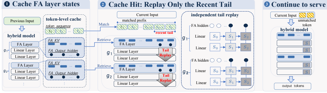
Figure 1: Tail-Replay overview: cache FA KV and FA output hiddens, independently applies Tail-Replay to each linear-attention group on a cache hit, and then process the unmatched suffix.
