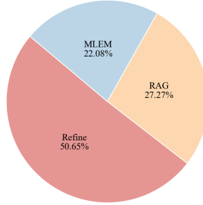
Fig. 2. Distribution of action types executed by RLEA on OR-Tools.
