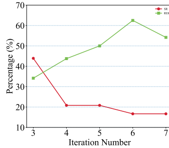
Fig. 3. Sensitivity analysis of OR-Tools performance relative to iterations
