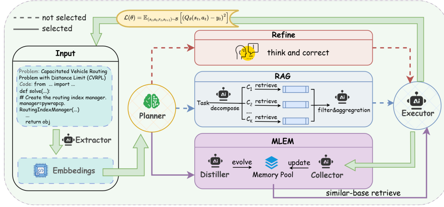
Fig. 1. Architecture of RLEA for automated VRP modeling. The input consists of the problem name and the current modeling code to be generated or revised. An extractor encodes this pair into embeddings, which define the Planner state. Based on the current state, the Planner follows a policy \pi(a | s) to select the action, such as exploiting similar historical experiences from the memory pool (MLEM). The selected action is then executed to generate or update the modeling code and invoke the solver for the current problem instance. During training, the Planner samples actions according to the learned policy; during inference, the Planner is frozen and selects actions deterministically.
