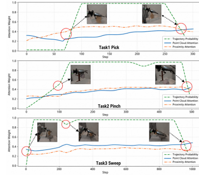
Figure 7: Attention visualization. Averaged Transformer attention weights of point-cloud and proximity tokens across three tabletop tasks.
