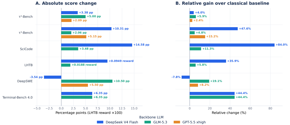
Figure 3 | Performance changes from classical baselines to QART hybrid models constructed with the same backbone LLM. The left panel shows absolute score changes, and the right panel shows relative gains over the corresponding classical baseline. Results are grouped by benchmark, with colors identifying the backbone LLM. Positive values favor the QART hybrid configuration; negative values indicate a regression. Missing bars denote combinations that were not evaluated. LHTB absolute changes are multiplied by 100 for bar length, while annotations retain native reward units.
