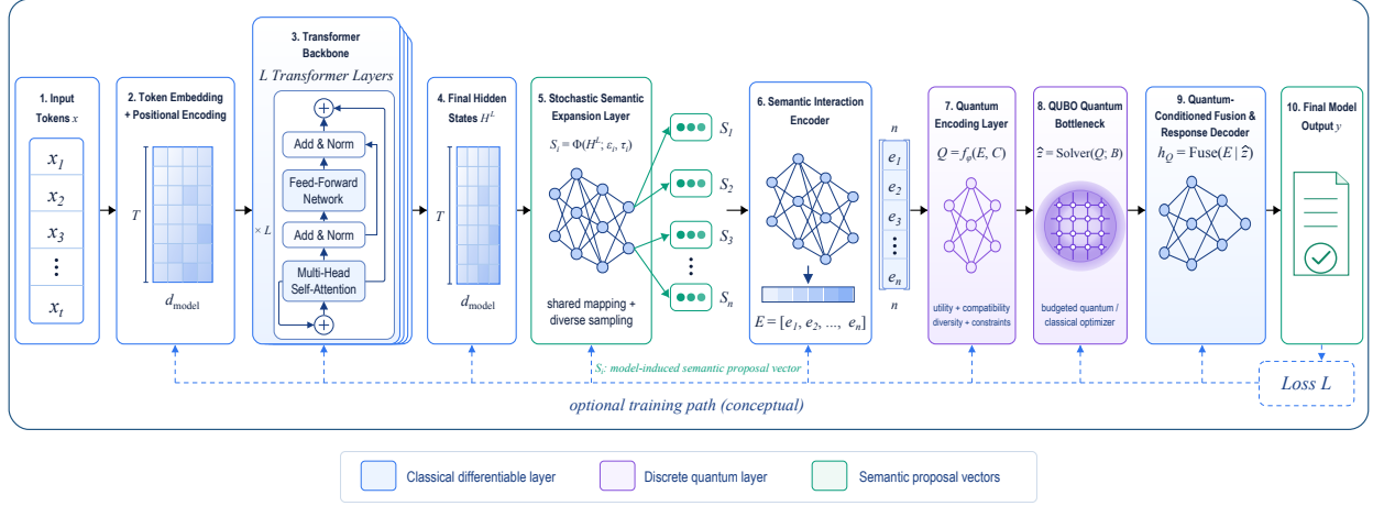
Figure 1 | Architectural design of QART, combining a Transformer language model with an optimization component in a quantum–classical hybrid architecture. The diagram is a conceptual hidden-representation route; an alternative model-generated-content interface y_h is described in Section 6. The solver returns a finite-budget candidate \hat{z} = \text{Solver}(Q; B) , while z^* \in \arg \min_z z^\top Q z remains the theoretical reference optimum. The accompanying description focuses on functional roles rather than proprietary implementation details.
