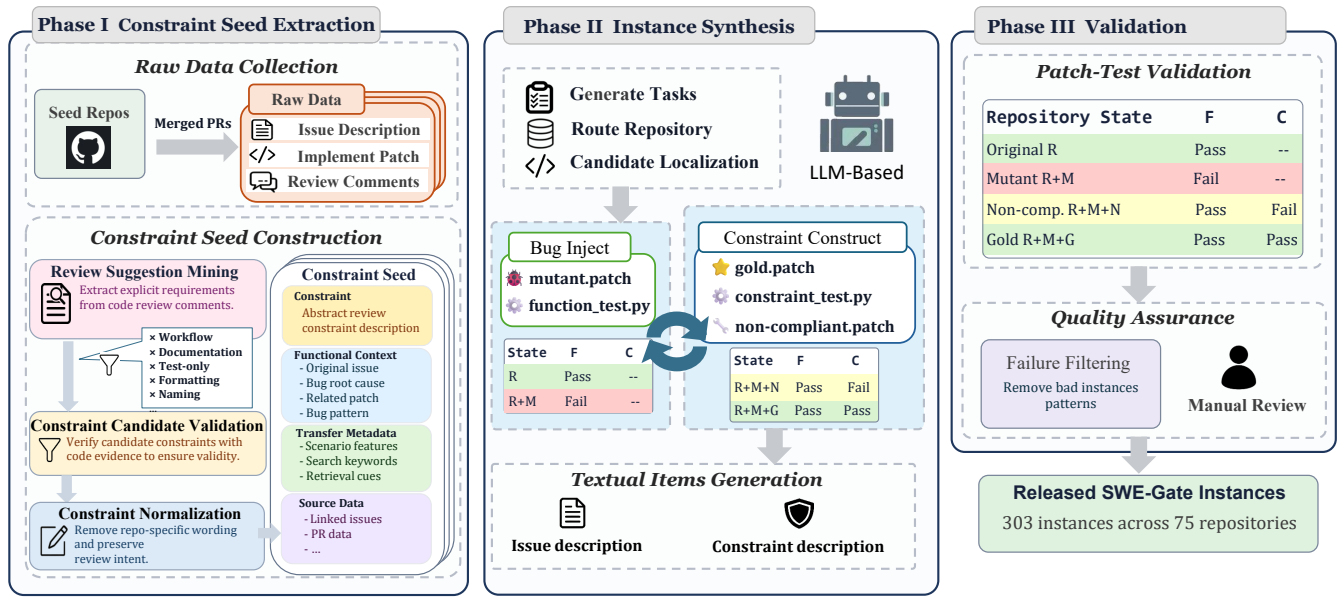
Figure 1: Overview of the SWE-Gate construction pipeline. SWE-Gate reconstructs issue-pull request artifacts, uses LLM-based processing to extract atomic review suggestions and select verifiable constraint seeds, transfers the seeds into compatible repository contexts, and validates the resulting instances through executable tests and quality assurance.
