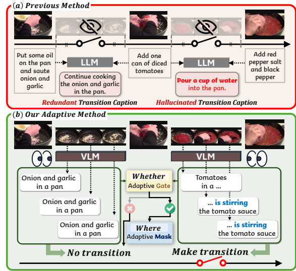
Figure 1: (a) Prior work (Kim et al., 2026) synthesizes captions from GT text alone, producing hallucinated descriptions (e.g., “pour a cup of water”) and rigidly bridging all gaps. (b) SBS generates visually grounded captions via VLM and selectively bridges gaps only when a genuine semantic transition is detected.
