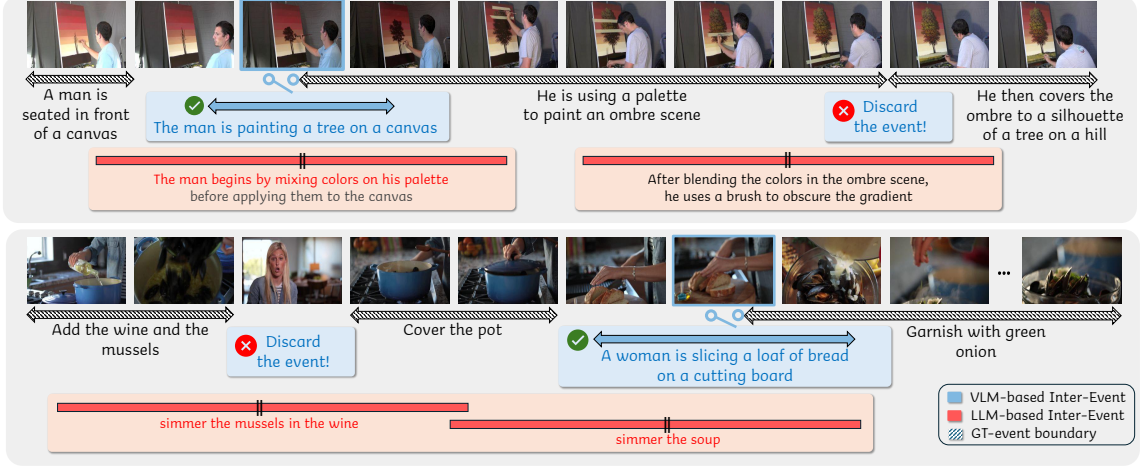
Figure 3: Qualitative results about transition events. Prior LLM-based method injects a transition into every gap, including uninformative ones. Also, even for meaningful transitions, they describe regions misaligned with the actual transition, resulting in inaccurate captions. In contrast, SBS generates transitions only where a meaningful change occurs, producing captions that are well aligned with both the actual transition and the underlying frames.
