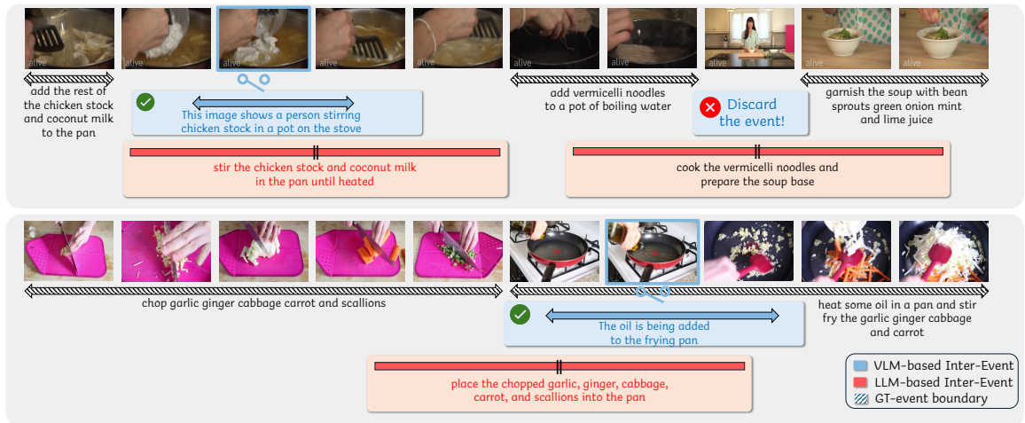
Figure A.2: Qualitative results about transition events on YouCook2.
