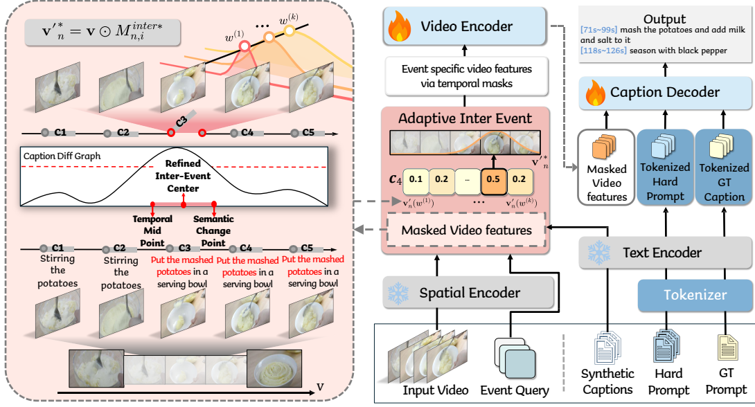
Figure 2: SBS Pipeline. Using VLM-generated frame captions as a visually grounded narrative flow, SBS decides whether to introduce a transition in each gap via an adaptive gate and where to place it via an adaptive mask, providing grounded auxiliary supervision.
