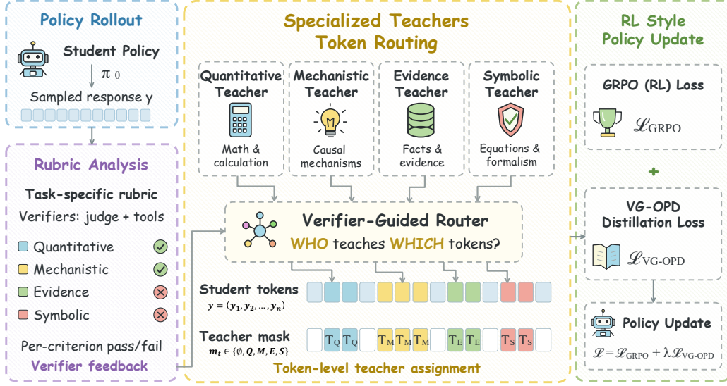
Figure 2: Overview of VG-OPD . The student’s rollouts are scored per criterion by the rubric’s verifiers; for each failed criterion, the expert of that criterion’s axis is licensed only if it answers better; the licensed teacher supervises only the tokens on which it disagrees with the student; the gated KL enters the GRPO update as an additive token-level advantage.
