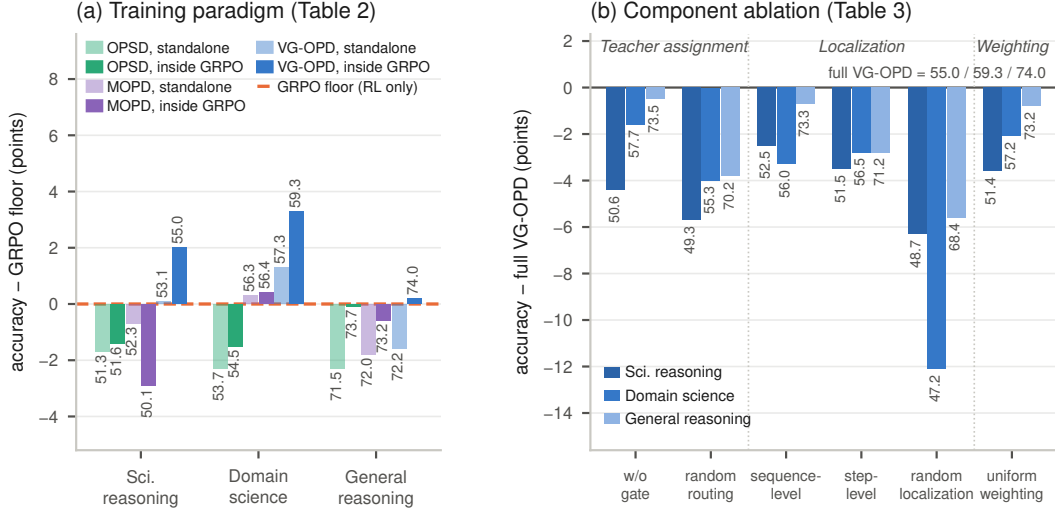
Figure 5: Tables 2 and 3 as differences. (a) Group-average accuracy of each distillation recipe relative to the RL-only GRPO floor (dashed line), standalone (light) and inside GRPO (solid); every bar is labelled with its absolute accuracy from Table 2. (b) Each ablation variant relative to full VG-OPD, one bar per benchmark group, labelled with the absolute accuracy from Table 3.
