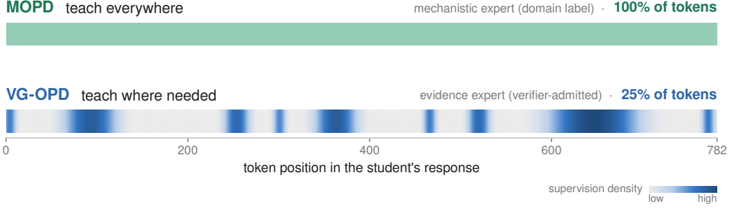
Figure 1: Who teaches which token? Token-level supervision comparison on one 782-token student rollout. MOPD applies dense supervision from a single domain teacher, while VG-OPD selectively assigns experts and concentrates supervision on tokens where the selected expert disagrees with the student. In this example, the evidence expert supervises only a subset of tokens, with darker spans indicating stronger supervision.
