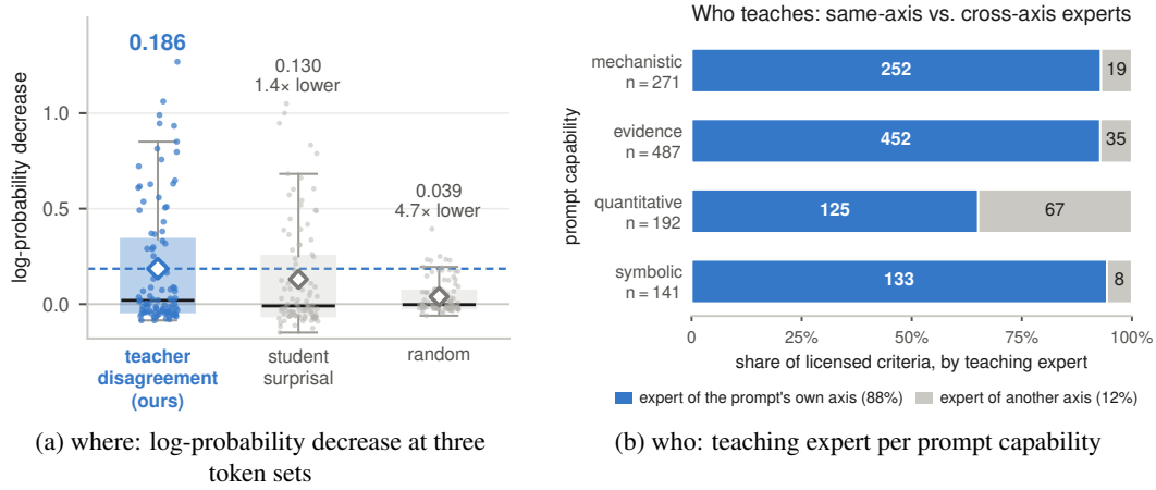
Figure 3: Mechanism analysis. (a) Decrease D_t in the starting model’s log-probability of its own tokens after training, per rollout, at teacher-disagreement, highest-surprisal, and random positions (box: IQR, line: median, diamond: mean). (b) Who teaches the licensed criteria: the prompt’s own-axis expert (blue) or another axis’s expert (grey) with counts in the bars.
