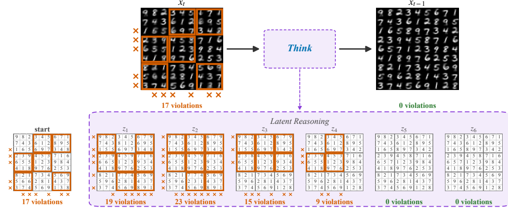
Figure 11: Latent reasoning within one denoising step, each recursion’s state \mathbf{z}_i decoded by a linear probe with violated constraints in orange. The Thinker introduces violations absent from \mathbf{x}_t and then resolves them, reaching a valid grid before anything is committed to \mathbf{x}_{t-1} .
