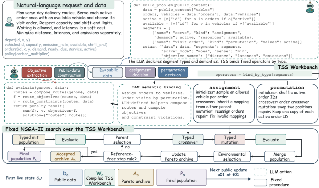
Figure 2: Constructing the initial state. The model builds W_0 from D_0 ; TSS and NSGA-II produce P_0 and A_0 . Dashed teal marks model-authored code; solid blue-gray marks fixed execution.
