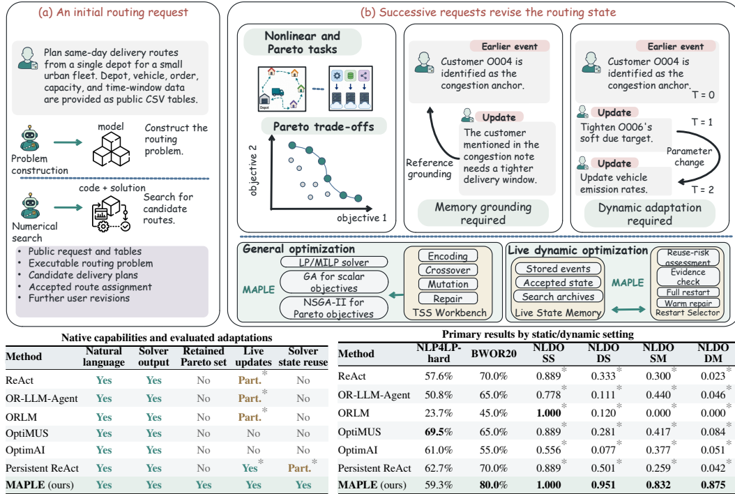
Figure 1: MAPLE maintains plans through successive requests. The routing example shows problem revision, memory of earlier decisions, and reuse of search results. The tables compare capabilities and performance. An asterisk marks adapted baselines.
