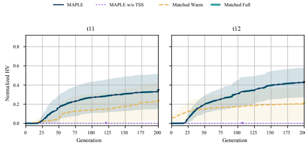
Figure 10: Recorded within-search behavior at disruptive routing updates. Ten-seed feasibility-gated HV means, standard-deviation bands, and mean stopping generations use the recorded reference. Figure 5 reports final quality under the fresh common public-formula references.
