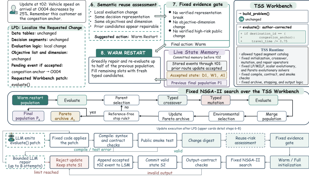
Figure 3: A localized routing update. LPD locates edits and LSM resolves historical references. Compilation and public-test errors trigger bounded repair; invalid search outputs reject the update. Valid outputs commit the state and history.
