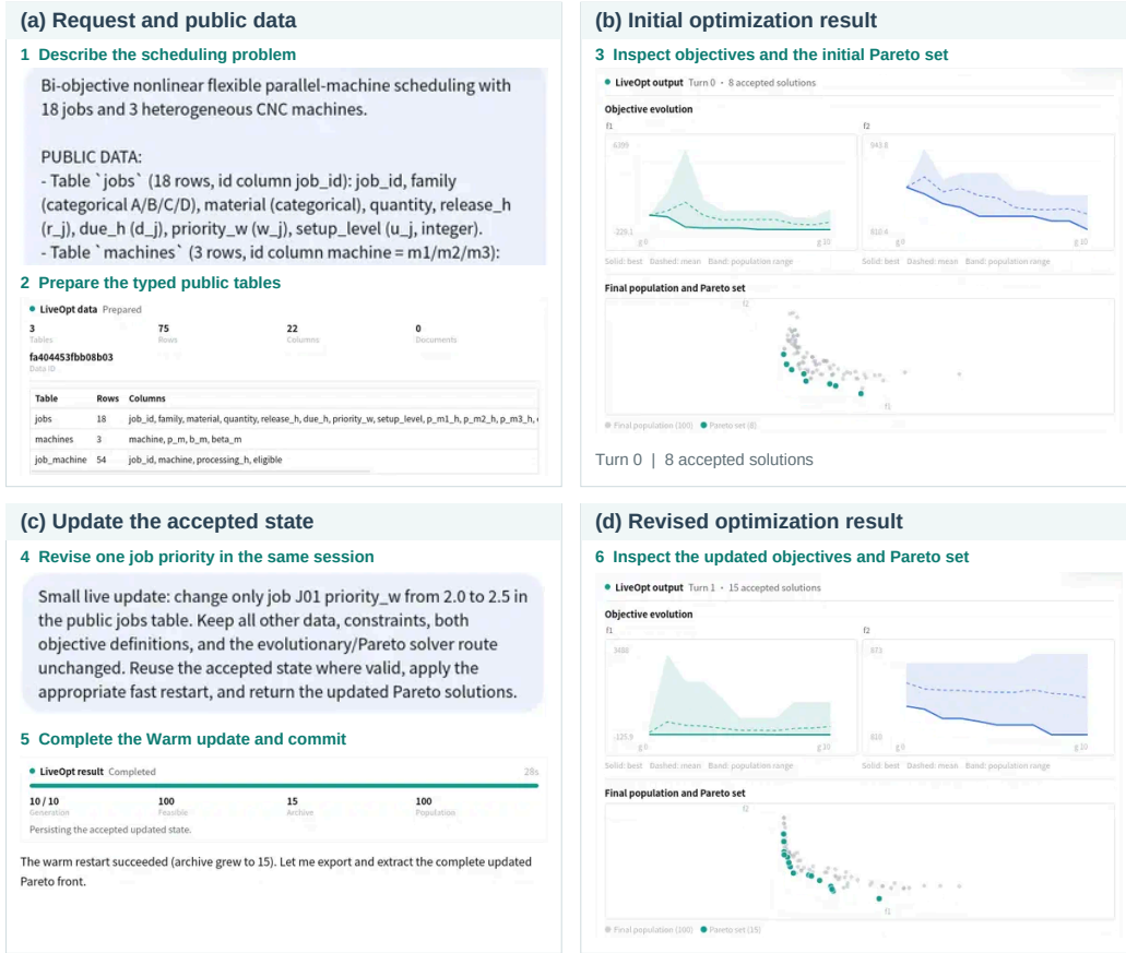
Figure 12: A complete Harness interaction from request to accepted update. Recorded steps: (a) scheduling request and public tables; (b) initial traces and eight Pareto solutions; (c) J01’s priority changes from 2.0 to 2.5, followed by a Warm update; (d) revised traces and fifteen Pareto solutions.
