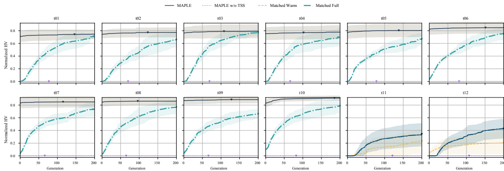
Figure 11: Green-routing component results (NLDO-P010, t01–t12). Recorded-evaluator mean HV over ten seeds, standard-deviation bands, and mean stopping generations (triangles). MAPLE and Matched Warm/Full remain feasible. Without TSS, duplicate vehicle assignment makes every P010 update infeasible with zero quality.
