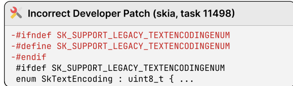
Figure 8: The developer patch incorrectly marked by ARVO for task 11498, which does not fix the root cause.
