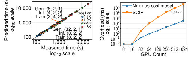
Figure 10. Cost-model fit to measured training-stage latency
