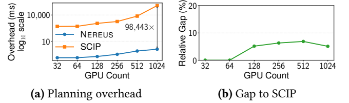
Figure 13. Transition planning across 32–1,024 GPUs.
