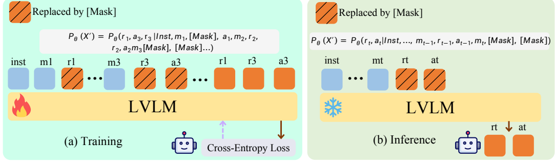
Figure 3: Overview of the MaP paradigm during training and inference.
