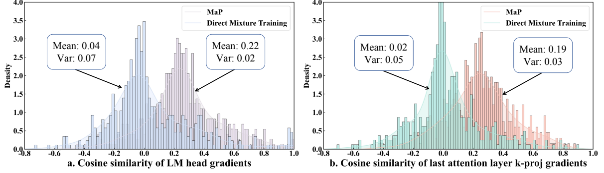
Figure 7: Kernel density estimation plots illustrating the gradient cosine similarity between individual training samples.
