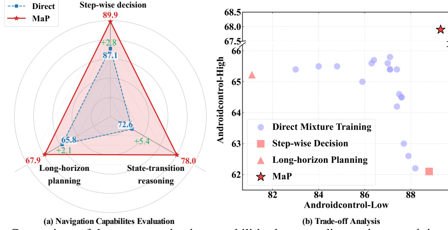
Figure 5: Left: Comparison of three core navigation capabilities between direct mixture training and MaP. Right: Trade-off analysis between direct mixture training and MaP.
