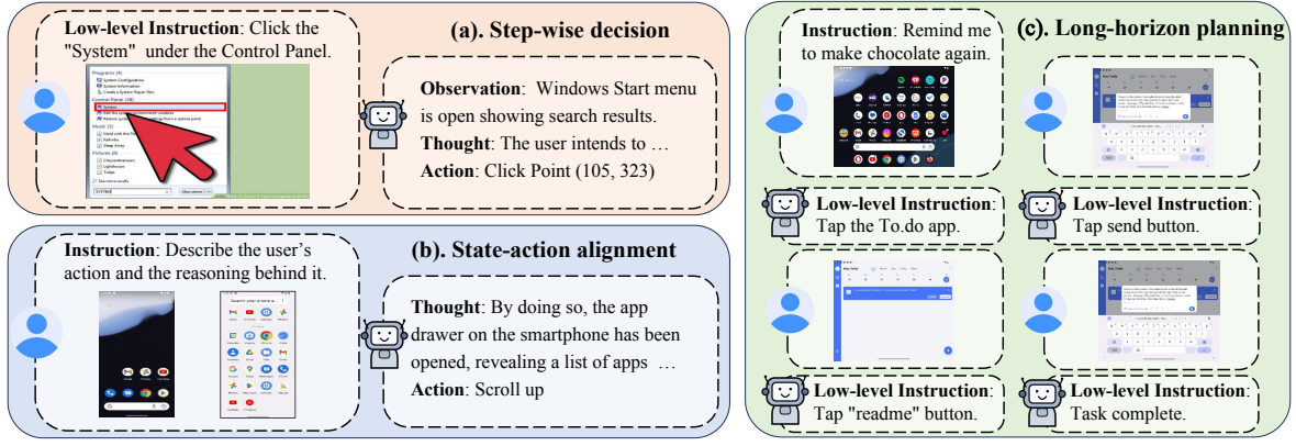
Figure 1: Overview of the three core dimensions of GUI navigation capabilities, which encompass (a) reasoning over current visual semantics, (b) understanding state-action alignment, and (c) maintaining long-horizon task consistency.
