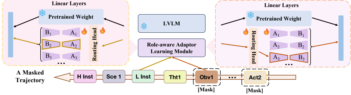
Figure 4: Illustration of the role-aware adapter learning module. Given a masked trajectory with heterogeneous components, the module dynamically assigns each token to a specific adapter for targeted optimization. Abbreviation: H Inst=High level instruction; L Inst=Low level instruction; Scene=Screenshot; Tht=Thought; Obv=Observation; Act=Action.
