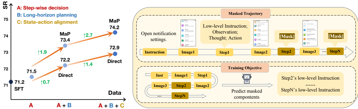
Figure 2: Left: Direct mixture training vs. MaP on the AndroidControl-High benchmark (Zhang et al., 2024). The \uparrow denotes the performance improvements over the single step-wise decision paradigm. Right: An overview of MaP. By masking arbitrary trajectory contents and predicting the counterparts, MaP unifies heterogeneous GUI corpora under a consistent training objective.
