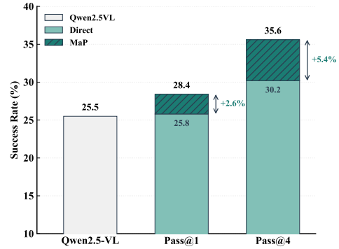
Figure 6: The performance of Qwen2.5VL-7B with direct mixture training and MaP on AndroidWorld.
