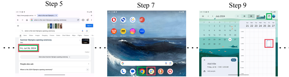
Figure 8: Qualitative results on the GUI-Odyssey dataset (Lu et al., 2024). High-level instructions are visualized at the top of each image. Predicted tap positions from our MaP (Qwen2.5-VL-3B) are shown in red, while those from the base model (Qwen2.5-VL-3B) are shown in green. Best viewed with zoom.
